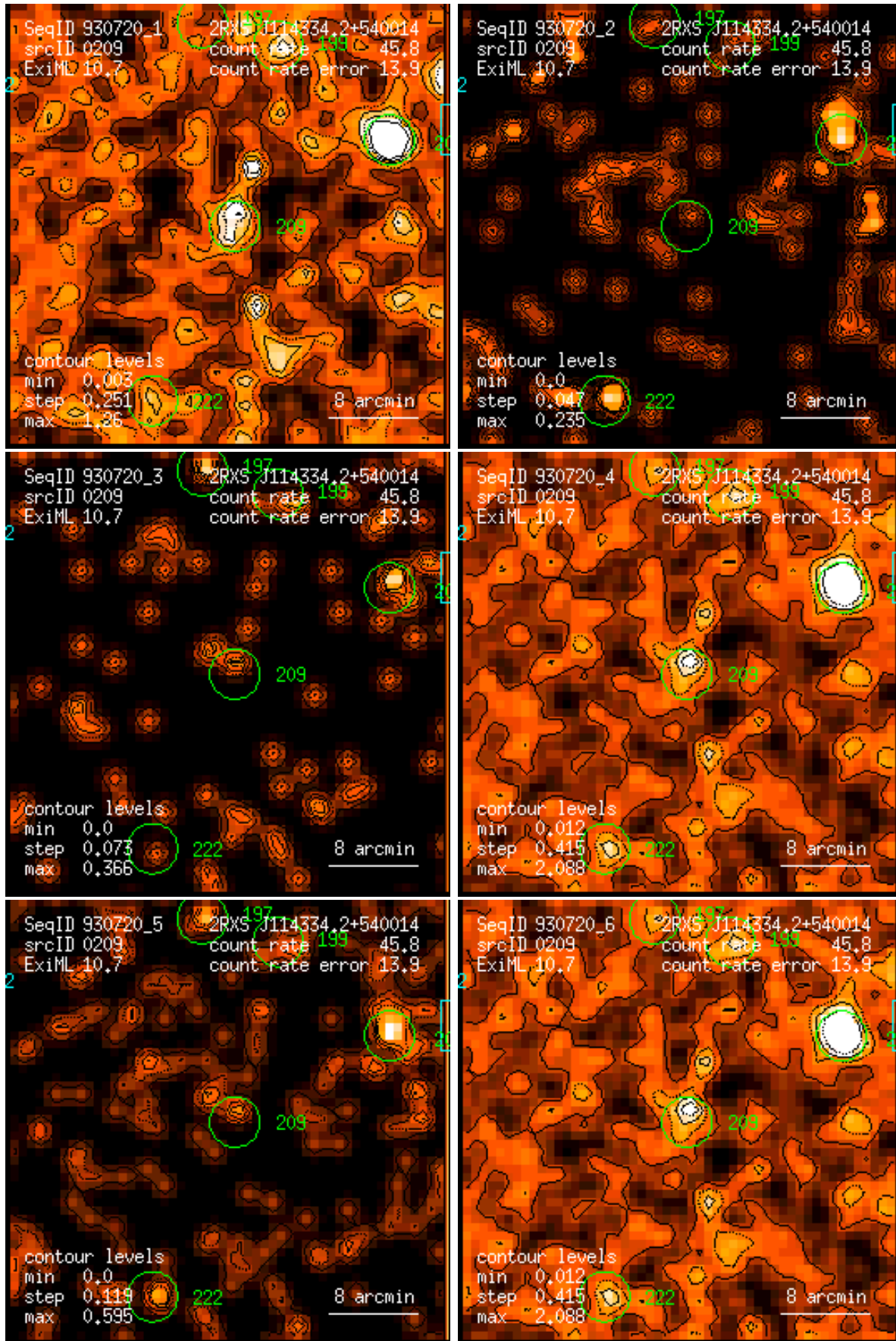
Figure 209: RASS 930720: detection 0209: band rate images, Gaussian filter: (1) PSPC channels 11 – 41, (2) 52 – 90, (3) 91 – 201, (4) 11 – 235, (5) 52 – 201, (6) 11 – 201. Broad band rates in counts/ks. Band rate contour levels in counts/ks/arcmin 2 .
