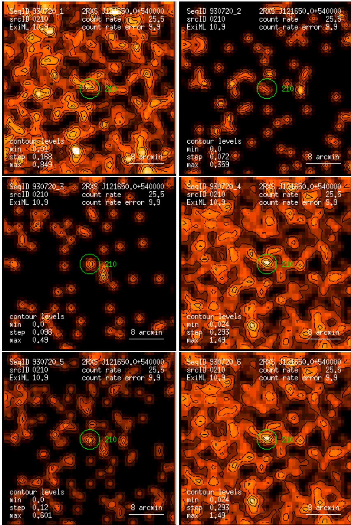
Figure 210: RASS 930720: detection 0210: band rate images, Gaussian filter: (1) PSPC channels 11 – 41, (2) 52 – 90, (3) 91 – 201, (4) 11 – 235, (5) 52 – 201, (6) 11 – 201. Broad band rates in counts/ks. Band rate contour levels in counts/ks/arcmin 2 .
