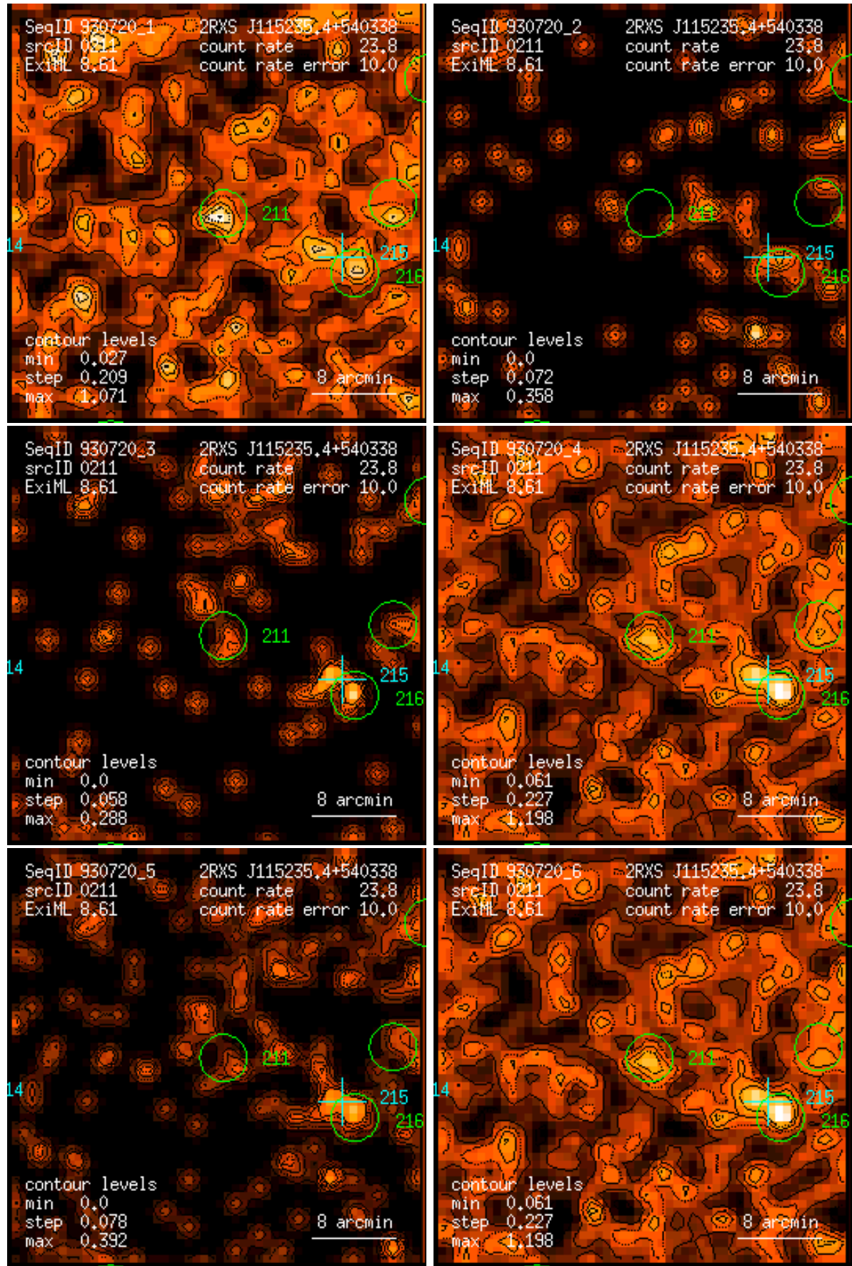
Figure 211: RASS 930720: detection 0211: band rate images, Gaussian filter: (1) PSPC channels 11 – 41, (2) 52 – 90, (3) 91 – 201, (4) 11 – 235, (5) 52 – 201, (6) 11 – 201. Broad band rates in counts/ks. Band rate contour levels in counts/ks/arcmin 2 .
