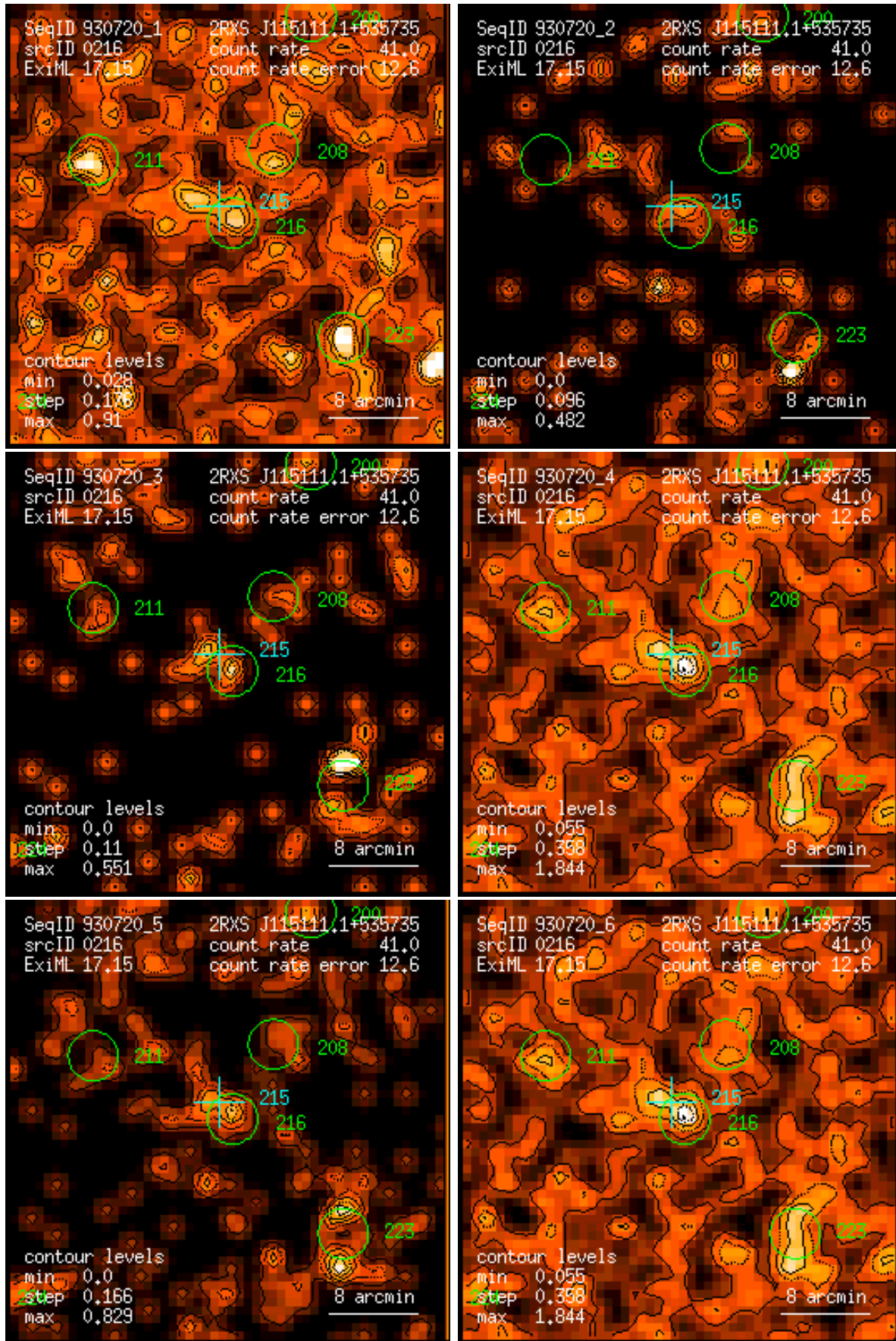
Figure 216: RASS 930720: detection 0216: band rate images, Gaussian filter: (1) PSPC channels 11 – 41, (2) 52 – 90, (3) 91 – 201, (4) 11 – 235, (5) 52 – 201, (6) 11 – 201. Broad band rates in counts/ks. Band rate contour levels in counts/ks/arcmin 2 .
