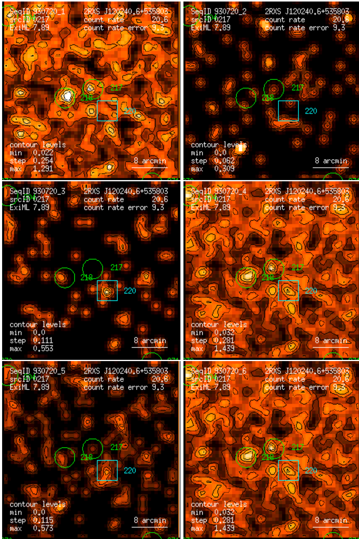
Figure 217: RASS 930720: detection 0217: band rate images, Gaussian filter: (1) PSPC channels 11 – 41, (2) 52 – 90, (3) 91 – 201, (4) 11 – 235, (5) 52 – 201, (6) 11 – 201. Broad band rates in counts/ks. Band rate contour levels in counts/ks/arcmin 2 .
