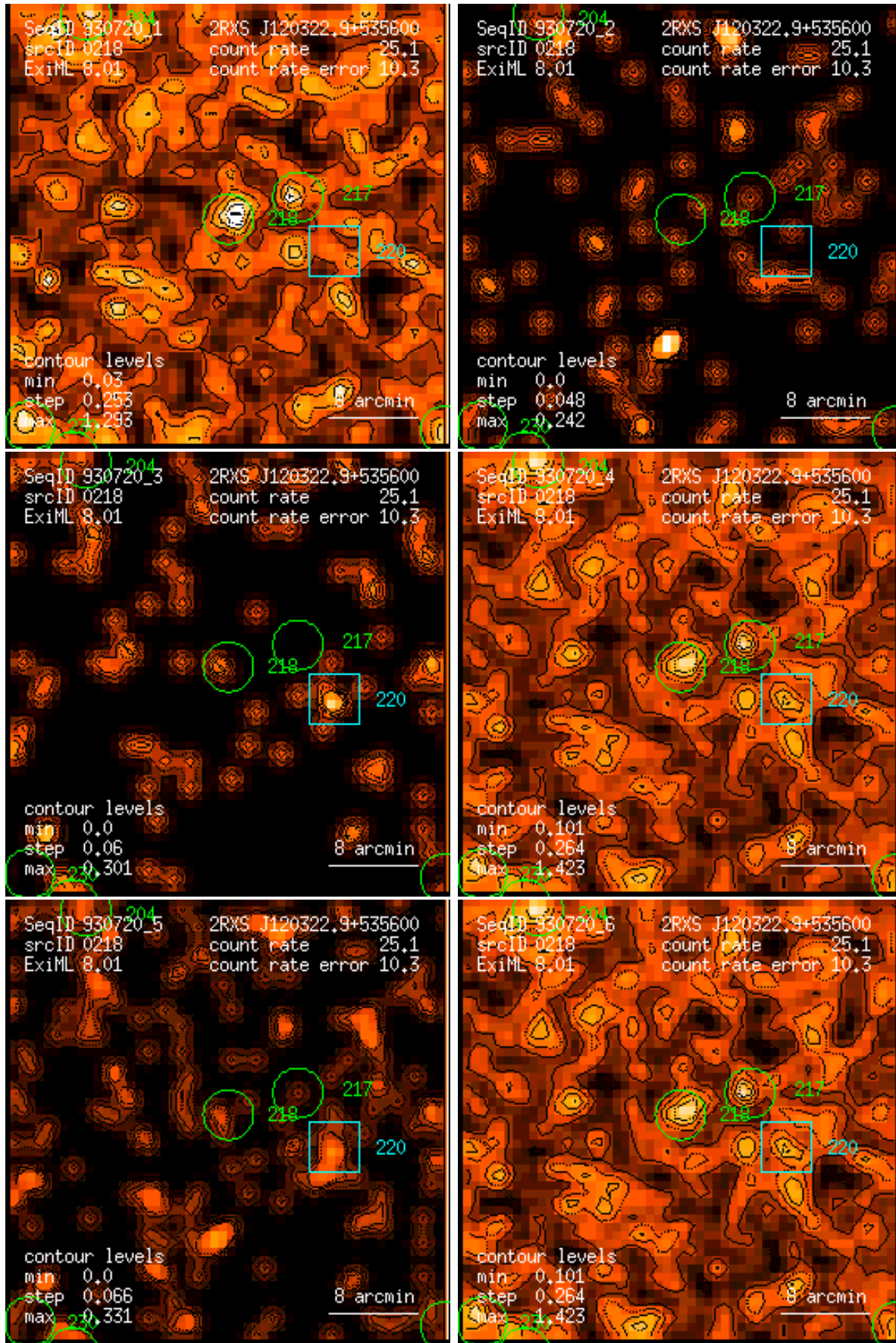
Figure 218: RASS 930720: detection 0218: band rate images, Gaussian filter: (1) PSPC channels 11 – 41, (2) 52 – 90, (3) 91 – 201, (4) 11 – 235, (5) 52 – 201, (6) 11 – 201. Broad band rates in counts/ks. Band rate contour levels in counts/ks/arcmin 2 .
