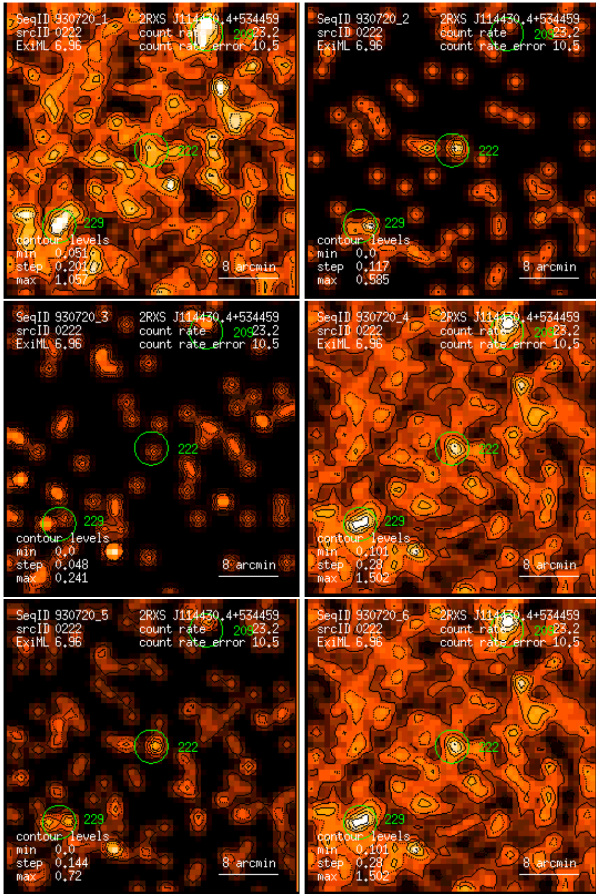
Figure 222: RASS 930720: detection 0222: band rate images, Gaussian filter: (1) PSPC channels 11 – 41, (2) 52 – 90, (3) 91 – 201, (4) 11 – 235, (5) 52 – 201, (6) 11 – 201. Broad band rates in counts/ks. Band rate contour levels in counts/ks/arcmin 2 .
