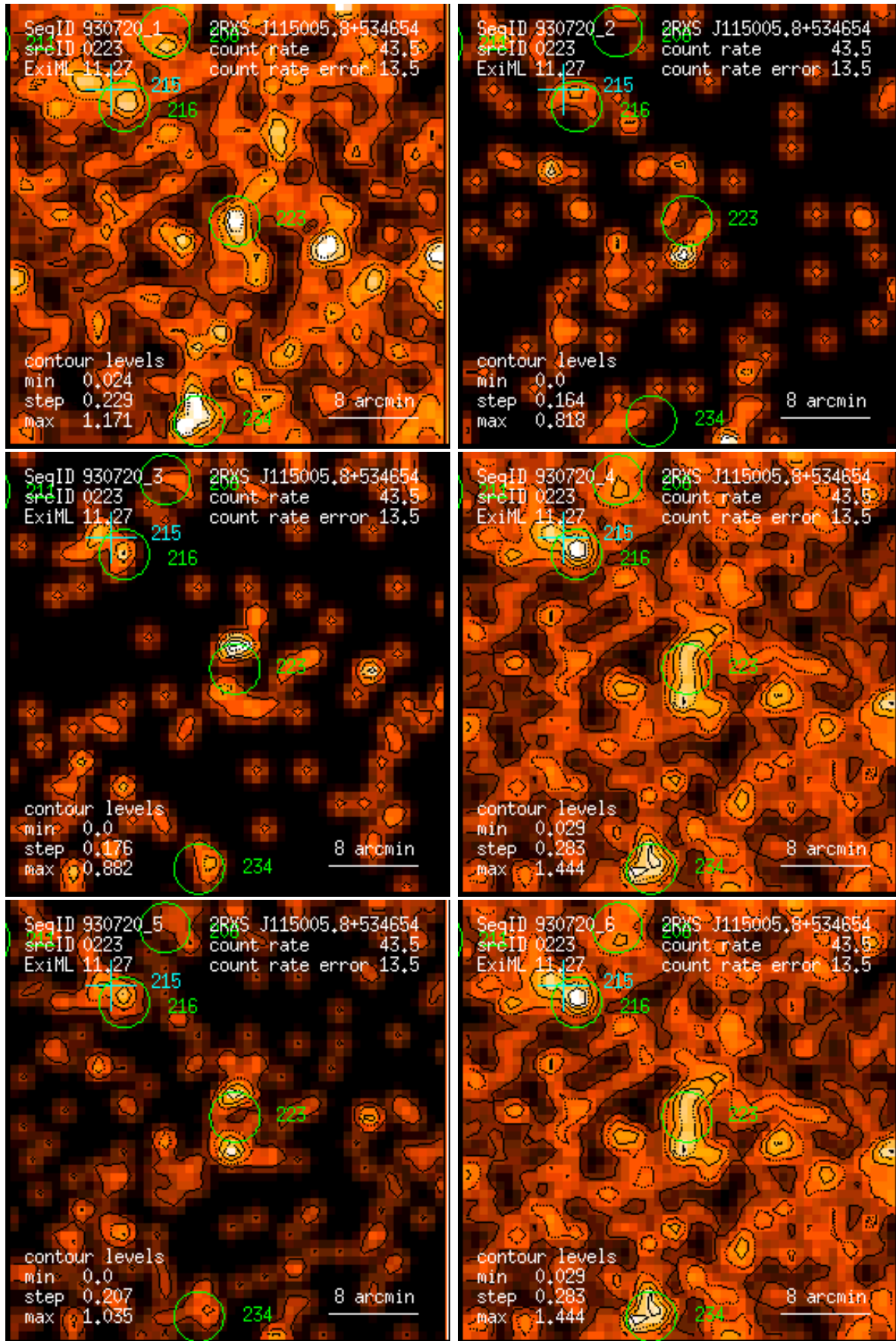
Figure 223: RASS 930720: detection 0223: band rate images, Gaussian filter: (1) PSPC channels 11 – 41, (2) 52 – 90, (3) 91 – 201, (4) 11 – 235, (5) 52 – 201, (6) 11 – 201. Broad band rates in counts/ks. Band rate contour levels in counts/ks/arcmin 2 .
