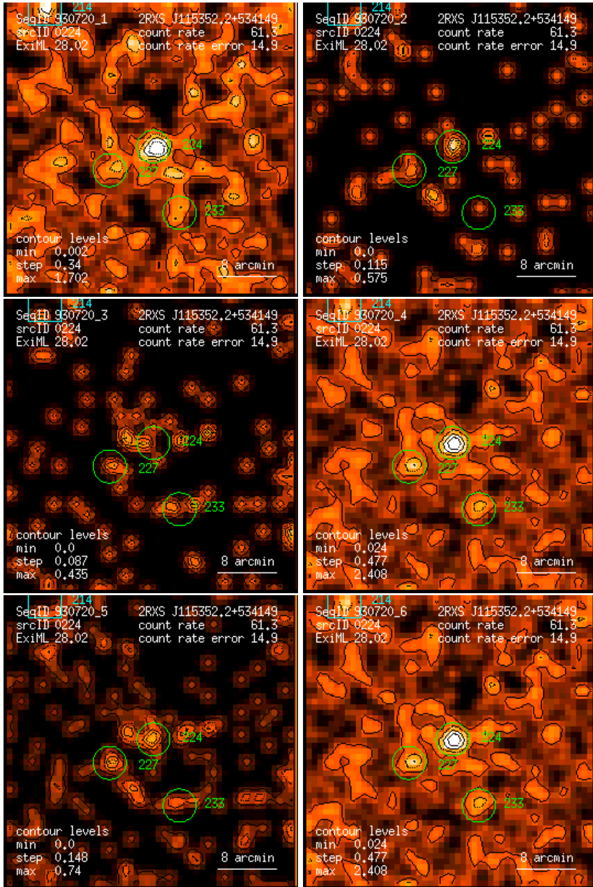
Figure 224: RASS 930720: detection 0224: band rate images, Gaussian filter: (1) PSPC channels 11 – 41, (2) 52 – 90, (3) 91 – 201, (4) 11 – 235, (5) 52 – 201, (6) 11 – 201. Broad band rates in counts/ks. Band rate contour levels in counts/ks/arcmin 2 .
