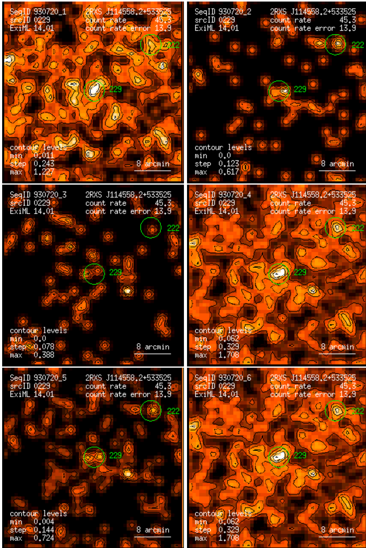
Figure 229: RASS 930720: detection 0229: band rate images, Gaussian filter: (1) PSPC channels 11 – 41, (2) 52 – 90, (3) 91 – 201, (4) 11 – 235, (5) 52 – 201, (6) 11 – 201. Broad band rates in counts/ks. Band rate contour levels in counts/ks/arcmin 2 .
