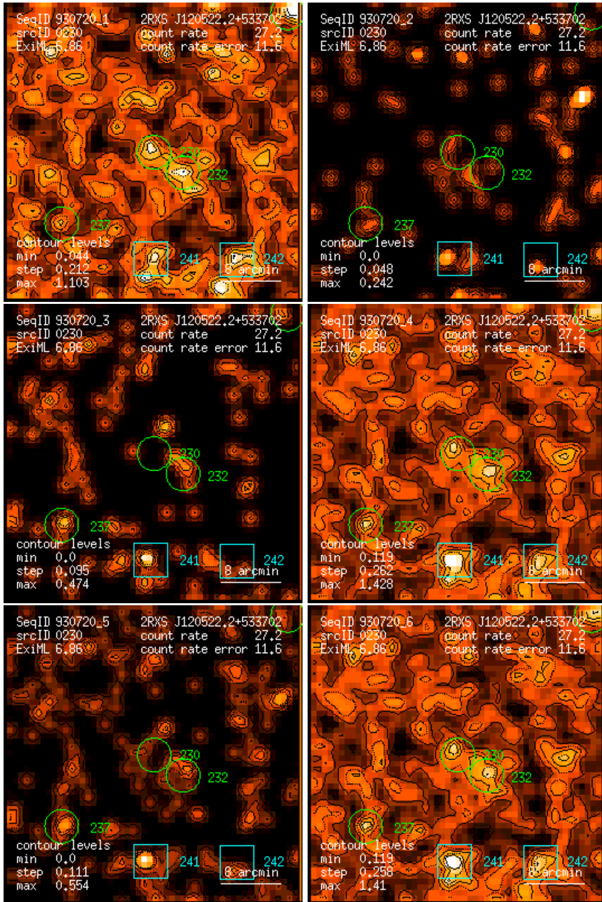
Figure 230: RASS 930720: detection 0230: band rate images, Gaussian filter: (1) PSPC channels 11 – 41, (2) 52 – 90, (3) 91 – 201, (4) 11 – 235, (5) 52 – 201, (6) 11 – 201. Broad band rates in counts/ks. Band rate contour levels in counts/ks/arcmin 2 .
