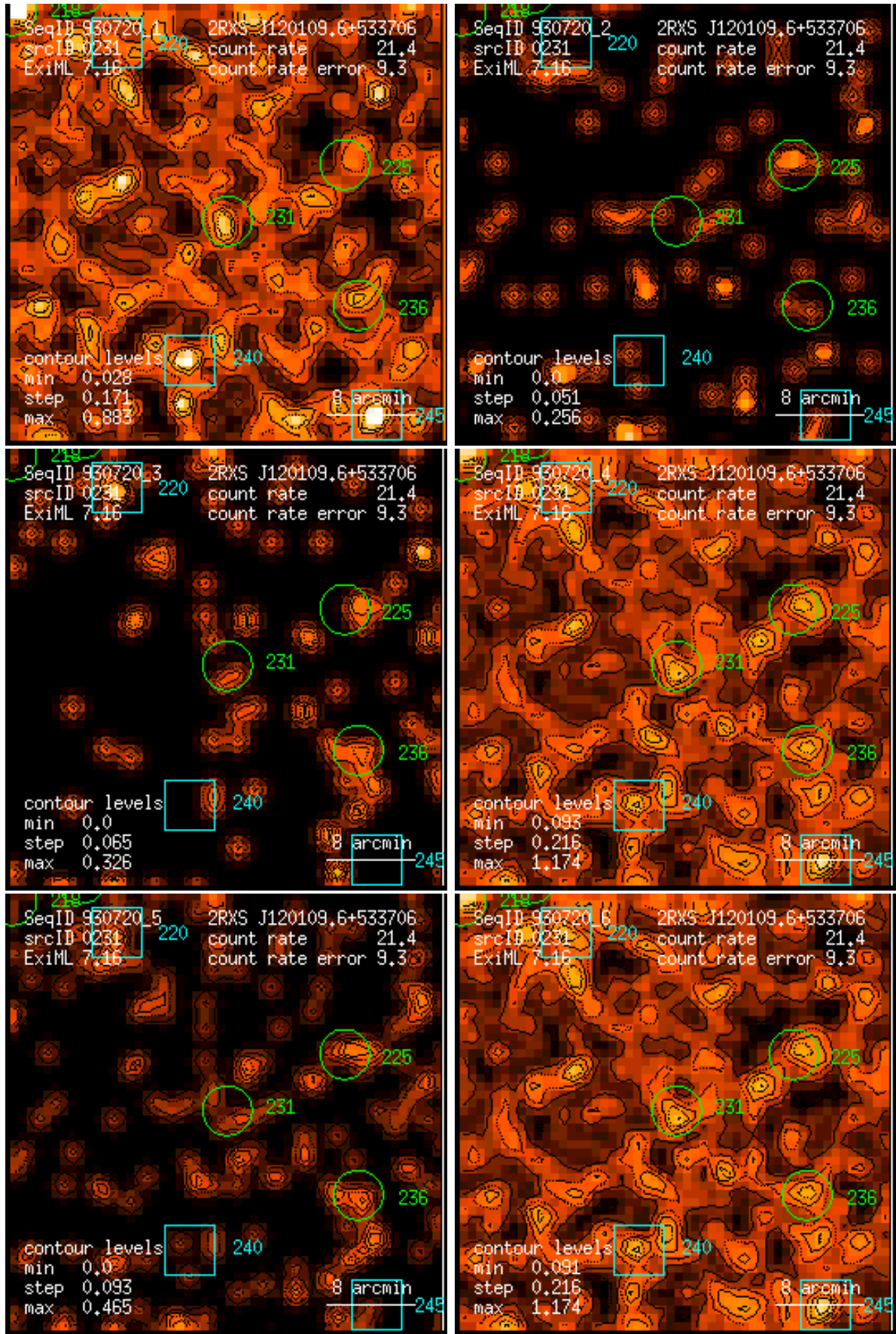
Figure 231: RASS 930720: detection 0231: band rate images, Gaussian filter: (1) PSPC channels 11 – 41, (2) 52 – 90, (3) 91 – 201, (4) 11 – 235, (5) 52 – 201, (6) 11 – 201. Broad band rates in counts/ks. Band rate contour levels in counts/ks/arcmin 2 .
