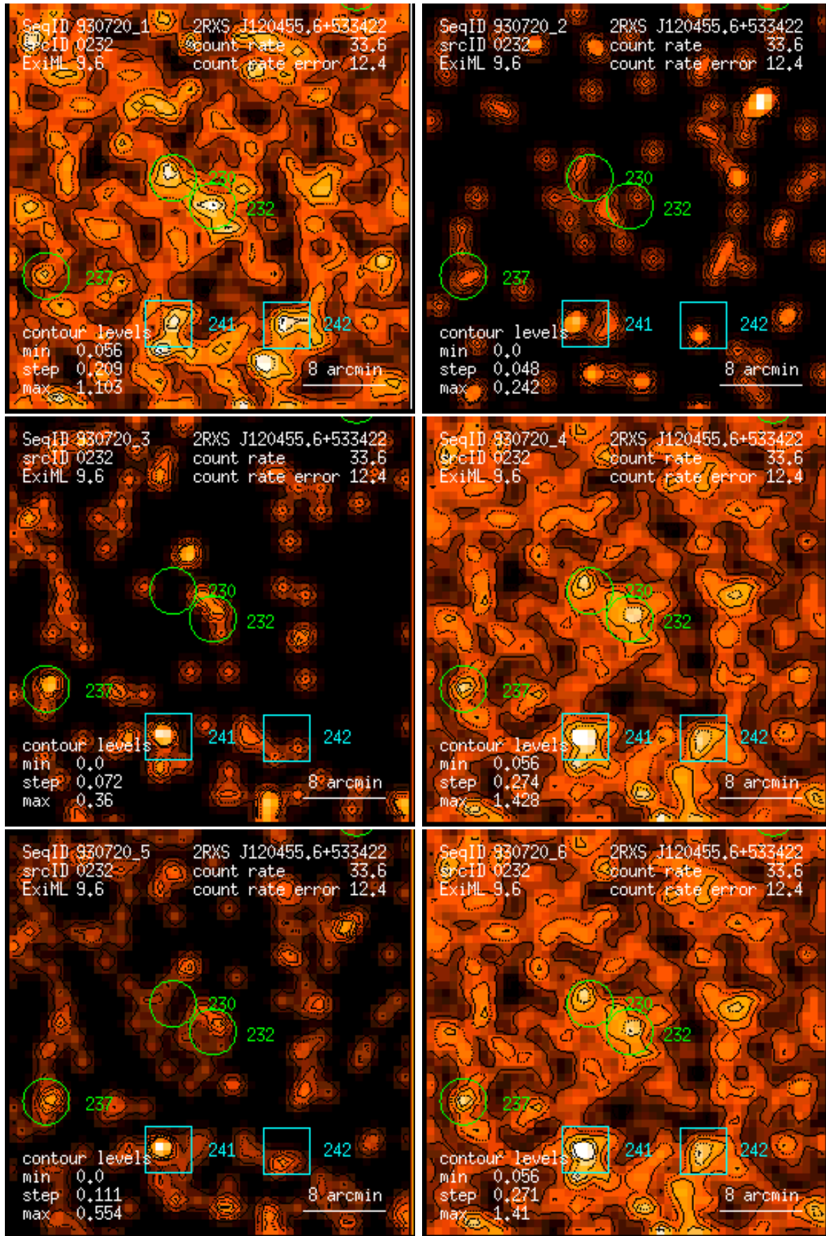
Figure 232: RASS 930720: detection 0232: band rate images, Gaussian filter: (1) PSPC channels 11 – 41, (2) 52 – 90, (3) 91 – 201, (4) 11 – 235, (5) 52 – 201, (6) 11 – 201. Broad band rates in counts/ks. Band rate contour levels in counts/ks/arcmin 2 .
