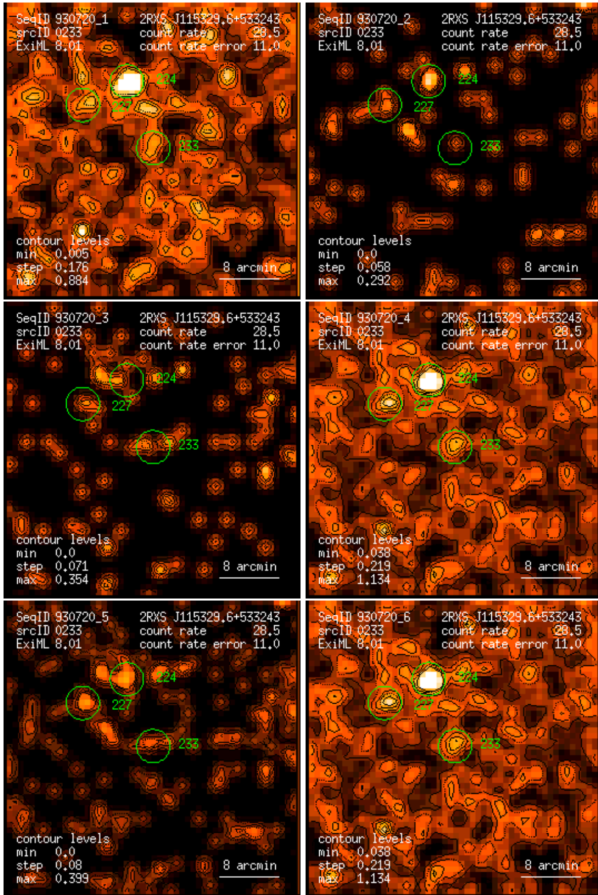
Figure 233: RASS 930720: detection 0233: band rate images, Gaussian filter: (1) PSPC channels 11 – 41, (2) 52 – 90, (3) 91 – 201, (4) 11 – 235, (5) 52 – 201, (6) 11 – 201. Broad band rates in counts/ks. Band rate contour levels in counts/ks/arcmin 2 .
