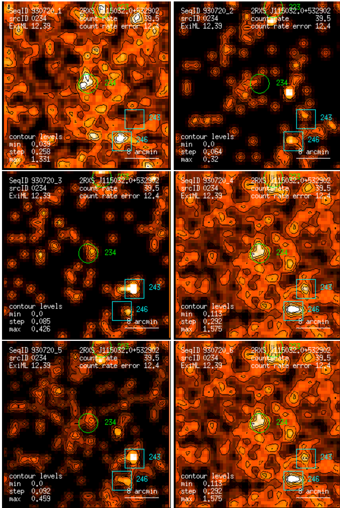
Figure 234: RASS 930720: detection 0234: band rate images, Gaussian filter: (1) PSPC channels 11 – 41, (2) 52 – 90, (3) 91 – 201, (4) 11 – 235, (5) 52 – 201, (6) 11 – 201. Broad band rates in counts/ks. Band rate contour levels in counts/ks/arcmin 2 .
