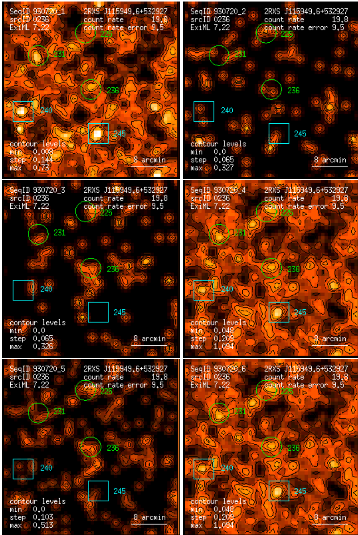
Figure 236: RASS 930720: detection 0236: band rate images, Gaussian filter: (1) PSPC channels 11 – 41, (2) 52 – 90, (3) 91 – 201, (4) 11 – 235, (5) 52 – 201, (6) 11 – 201. Broad band rates in counts/ks. Band rate contour levels in counts/ks/arcmin 2 .
