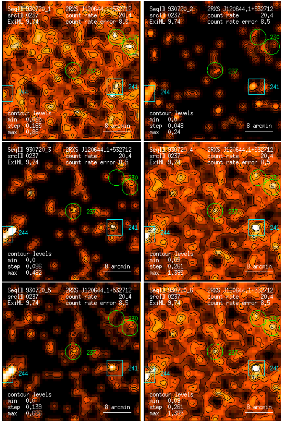
Figure 237: RASS 930720: detection 0237: band rate images, Gaussian filter: (1) PSPC channels 11 – 41, (2) 52 – 90, (3) 91 – 201, (4) 11 – 235, (5) 52 – 201, (6) 11 – 201. Broad band rates in counts/ks. Band rate contour levels in counts/ks/arcmin 2 .
