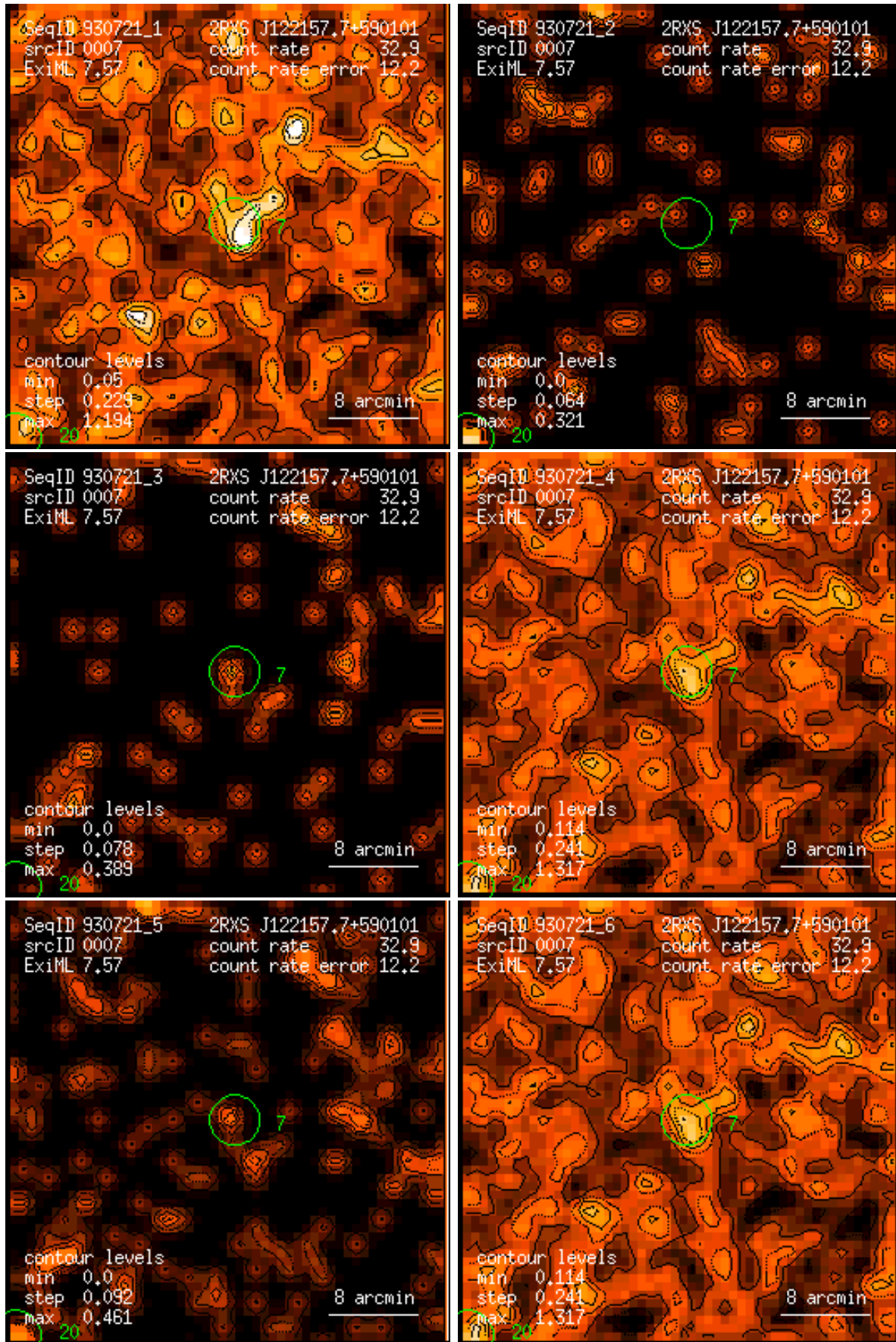
Figure 7: RASS 930721: detection 0007: band rate images, Gaussian filter: (1) PSPC channels 11 – 41, (2) 52 – 90, (3) 91 – 201, (4) 11 – 235, (5) 52 – 201, (6) 11 – 201. Broad band rates in counts/ks. Band rate contour levels in counts/ks/arcmin 2 .
