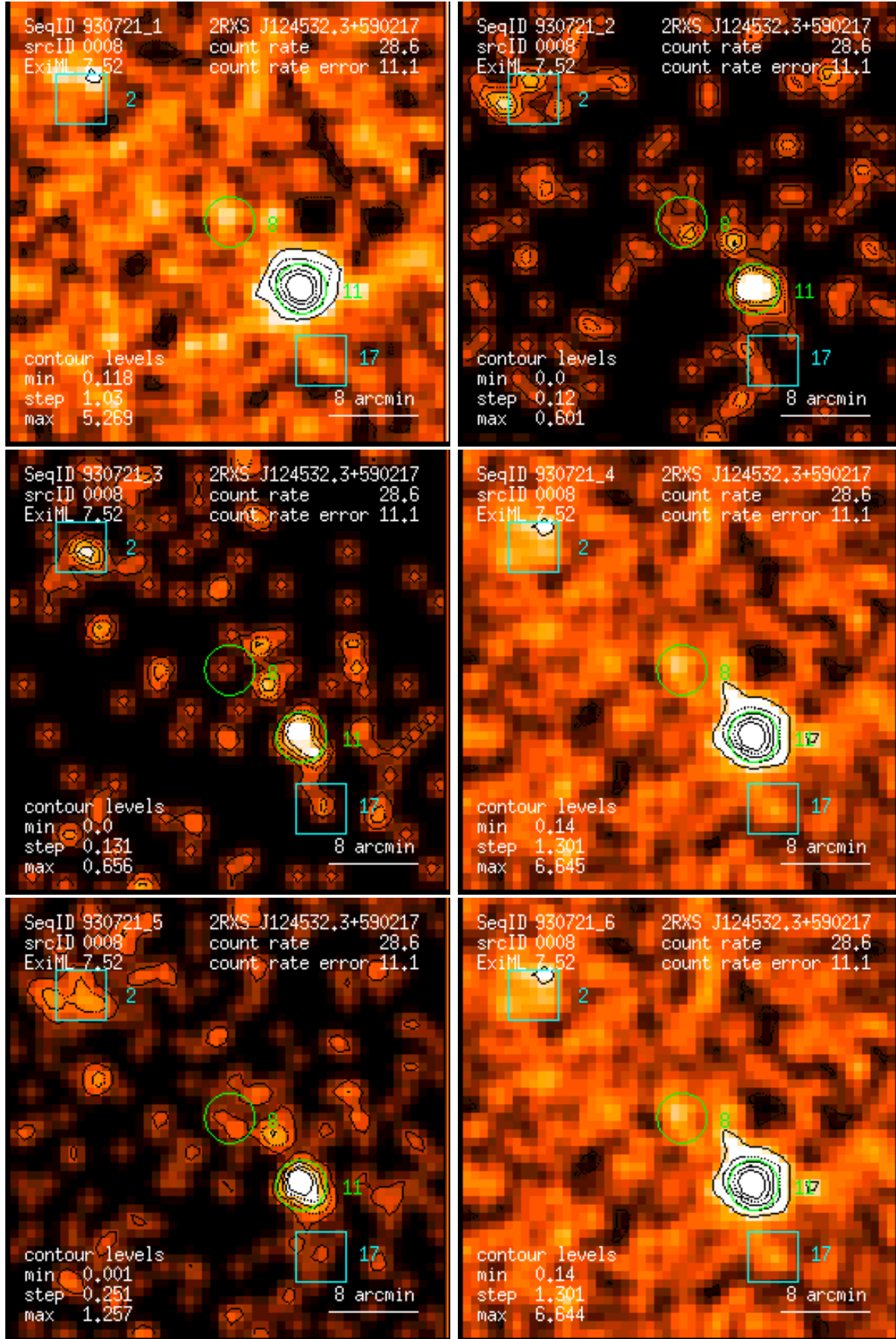
Figure 8: RASS 930721: detection 0008: band rate images, Gaussian filter: (1) PSPC channels 11 – 41, (2) 52 – 90, (3) 91 – 201, (4) 11 – 235, (5) 52 – 201, (6) 11 – 201. Broad band rates in counts/ks. Band rate contour levels in counts/ks/arcmin 2 .
