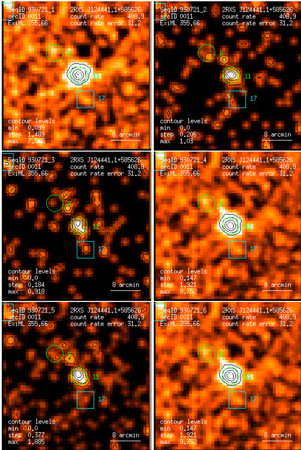
Figure 11: RASS 930721: detection 0011: band rate images, Gaussian filter: (1) PSPC channels 11 – 41, (2) 52 – 90, (3) 91 – 201, (4) 11 – 235, (5) 52 – 201, (6) 11 – 201. Broad band rates in counts/ks. Band rate contour levels in counts/ks/arcmin 2 .
