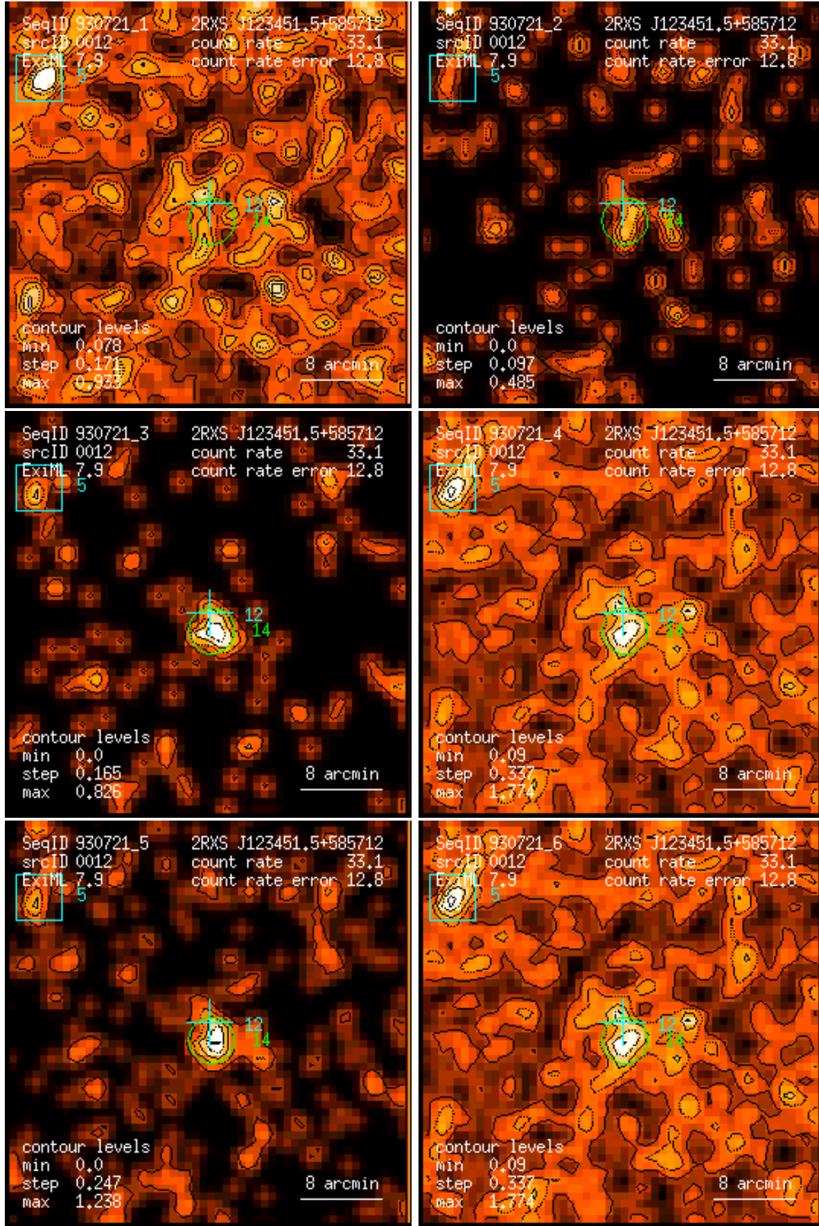
Figure 12: RASS 930721: detection 0012: band rate images, Gaussian filter: (1) PSPC channels 11 – 41, (2) 52 – 90, (3) 91 – 201, (4) 11 – 235, (5) 52 – 201, (6) 11 – 201. Broad band rates in counts/ks. Band rate contour levels in counts/ks/arcmin 2 .
