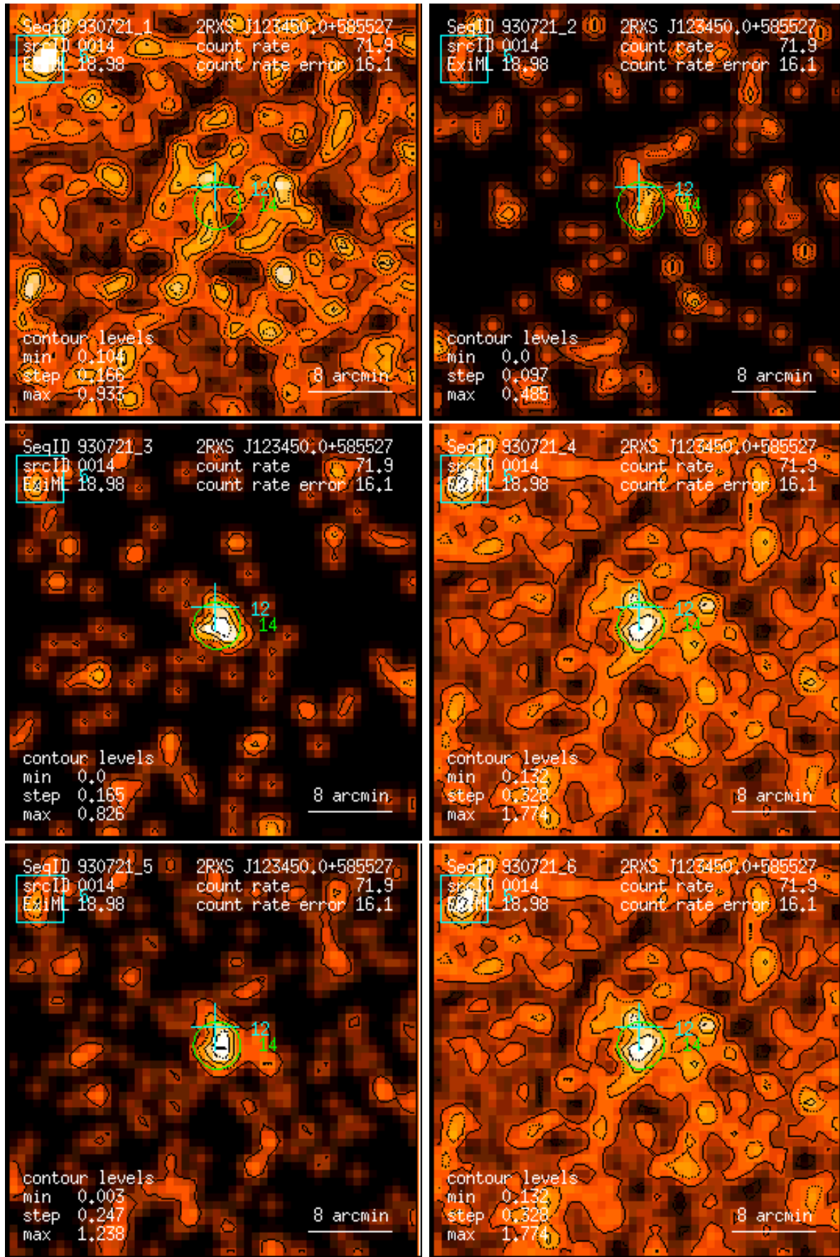
Figure 14: RASS 930721: detection 0014: band rate images, Gaussian filter: (1) PSPC channels 11 – 41, (2) 52 – 90, (3) 91 – 201, (4) 11 – 235, (5) 52 – 201, (6) 11 – 201. Broad band rates in counts/ks. Band rate contour levels in counts/ks/arcmin 2 .
