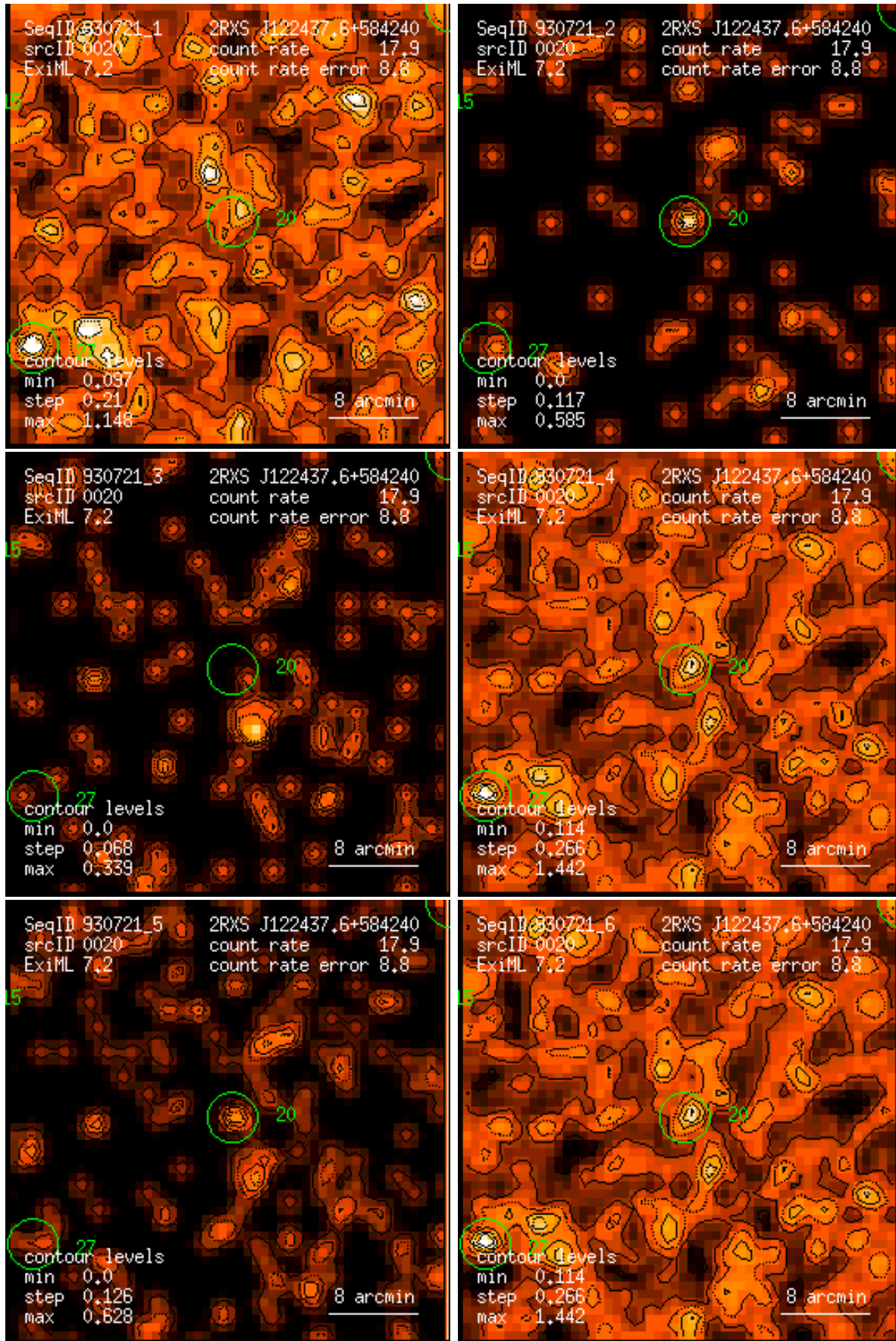
Figure 20: RASS 930721: detection 0020: band rate images, Gaussian filter: (1) PSPC channels 11 – 41, (2) 52 – 90, (3) 91 – 201, (4) 11 – 235, (5) 52 – 201, (6) 11 – 201. Broad band rates in counts/ks. Band rate contour levels in counts/ks/arcmin 2 .
