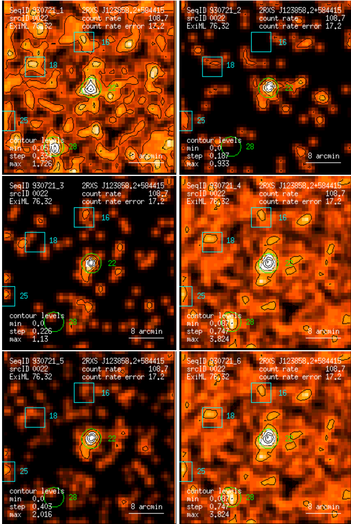
Figure 22: RASS 930721: detection 0022: band rate images, Gaussian filter: (1) PSPC channels 11 – 41, (2) 52 – 90, (3) 91 – 201, (4) 11 – 235, (5) 52 – 201, (6) 11 – 201. Broad band rates in counts/ks. Band rate contour levels in counts/ks/arcmin 2 .
