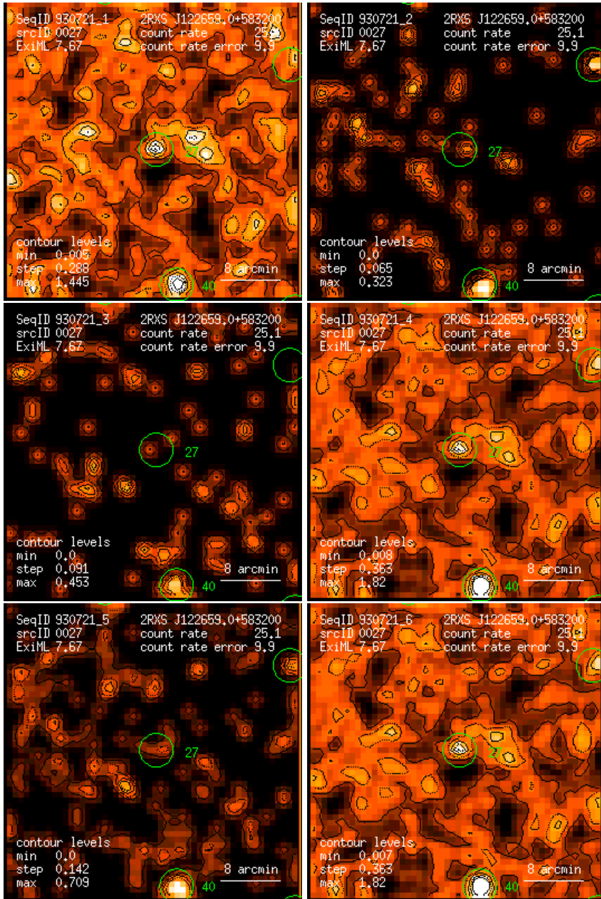
Figure 27: RASS 930721: detection 0027: band rate images, Gaussian filter: (1) PSPC channels 11 – 41, (2) 52 – 90, (3) 91 – 201, (4) 11 – 235, (5) 52 – 201, (6) 11 – 201. Broad band rates in counts/ks. Band rate contour levels in counts/ks/arcmin 2 .
