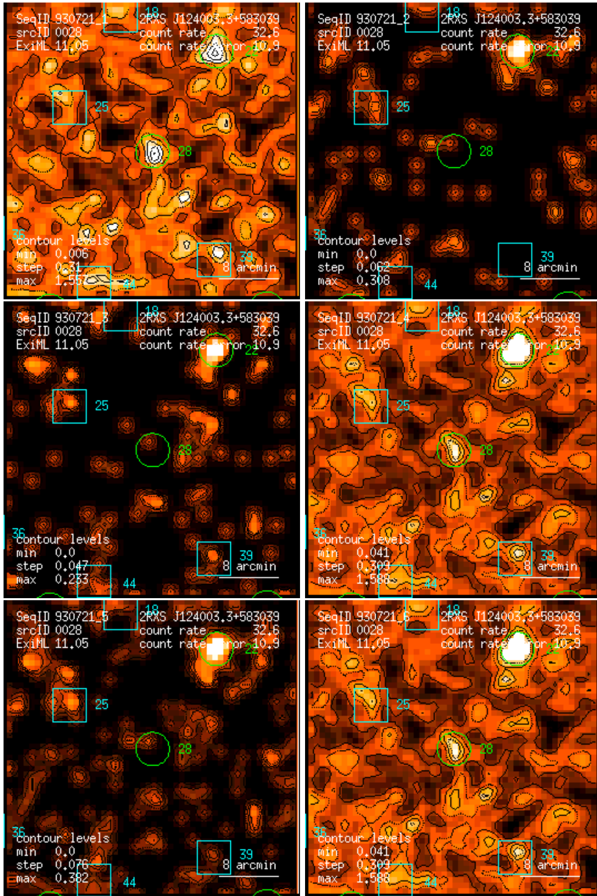
Figure 28: RASS 930721: detection 0028: band rate images, Gaussian filter: (1) PSPC channels 11 – 41, (2) 52 – 90, (3) 91 – 201, (4) 11 – 235, (5) 52 – 201, (6) 11 – 201. Broad band rates in counts/ks. Band rate contour levels in counts/ks/arcmin 2 .
