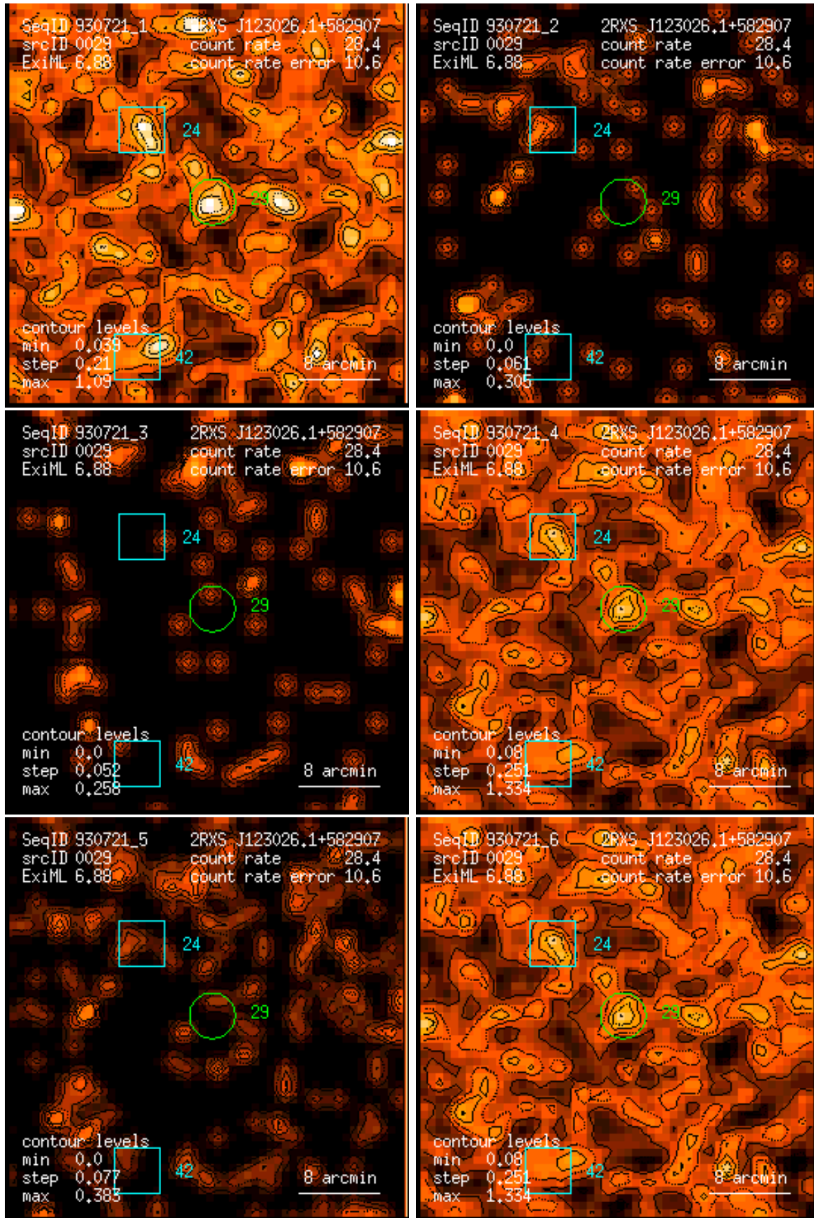
Figure 29: RASS 930721: detection 0029: band rate images, Gaussian filter: (1) PSPC channels 11 – 41, (2) 52 – 90, (3) 91 – 201, (4) 11 – 235, (5) 52 – 201, (6) 11 – 201. Broad band rates in counts/ks. Band rate contour levels in counts/ks/arcmin 2 .
