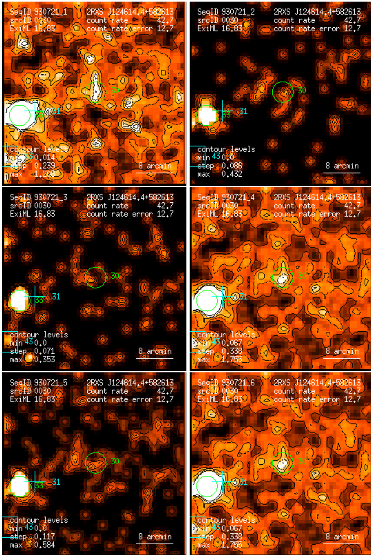
Figure 30: RASS 930721: detection 0030: band rate images, Gaussian filter: (1) PSPC channels 11 – 41, (2) 52 – 90, (3) 91 – 201, (4) 11 – 235, (5) 52 – 201, (6) 11 – 201. Broad band rates in counts/ks. Band rate contour levels in counts/ks/arcmin 2 .
