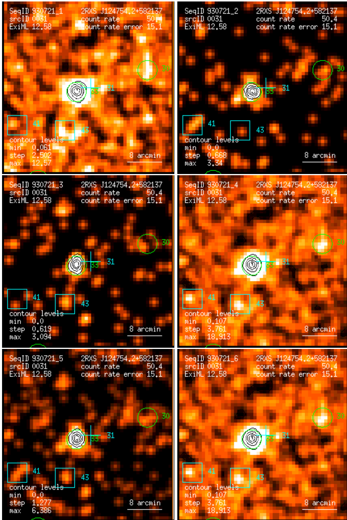
Figure 31: RASS 930721: detection 0031: band rate images, Gaussian filter: (1) PSPC channels 11 – 41, (2) 52 – 90, (3) 91 – 201, (4) 11 – 235, (5) 52 – 201, (6) 11 – 201. Broad band rates in counts/ks. Band rate contour levels in counts/ks/arcmin 2 .
