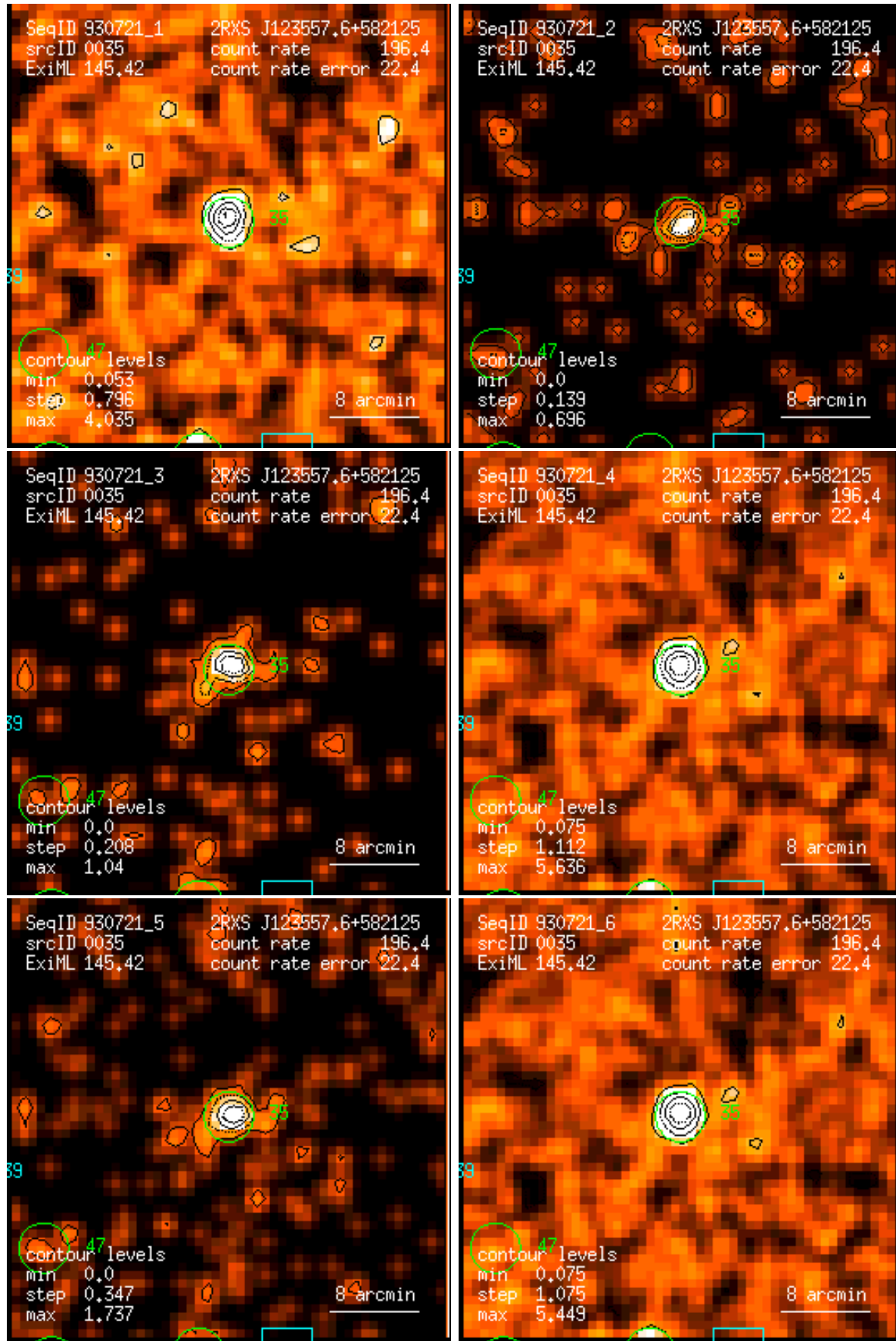
Figure 35: RASS 930721: detection 0035: band rate images, Gaussian filter: (1) PSPC channels 11 – 41, (2) 52 – 90, (3) 91 – 201, (4) 11 – 235, (5) 52 – 201, (6) 11 – 201. Broad band rates in counts/ks. Band rate contour levels in counts/ks/arcmin 2 .
