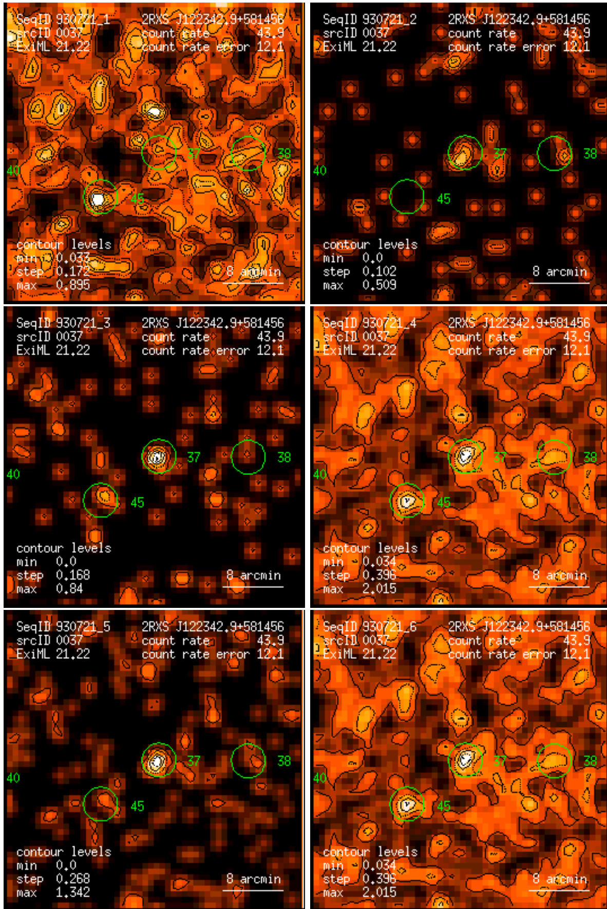
Figure 37: RASS 930721: detection 0037: band rate images, Gaussian filter: (1) PSPC channels 11 – 41, (2) 52 – 90, (3) 91 – 201, (4) 11 – 235, (5) 52 – 201, (6) 11 – 201. Broad band rates in counts/ks. Band rate contour levels in counts/ks/arcmin 2 .
