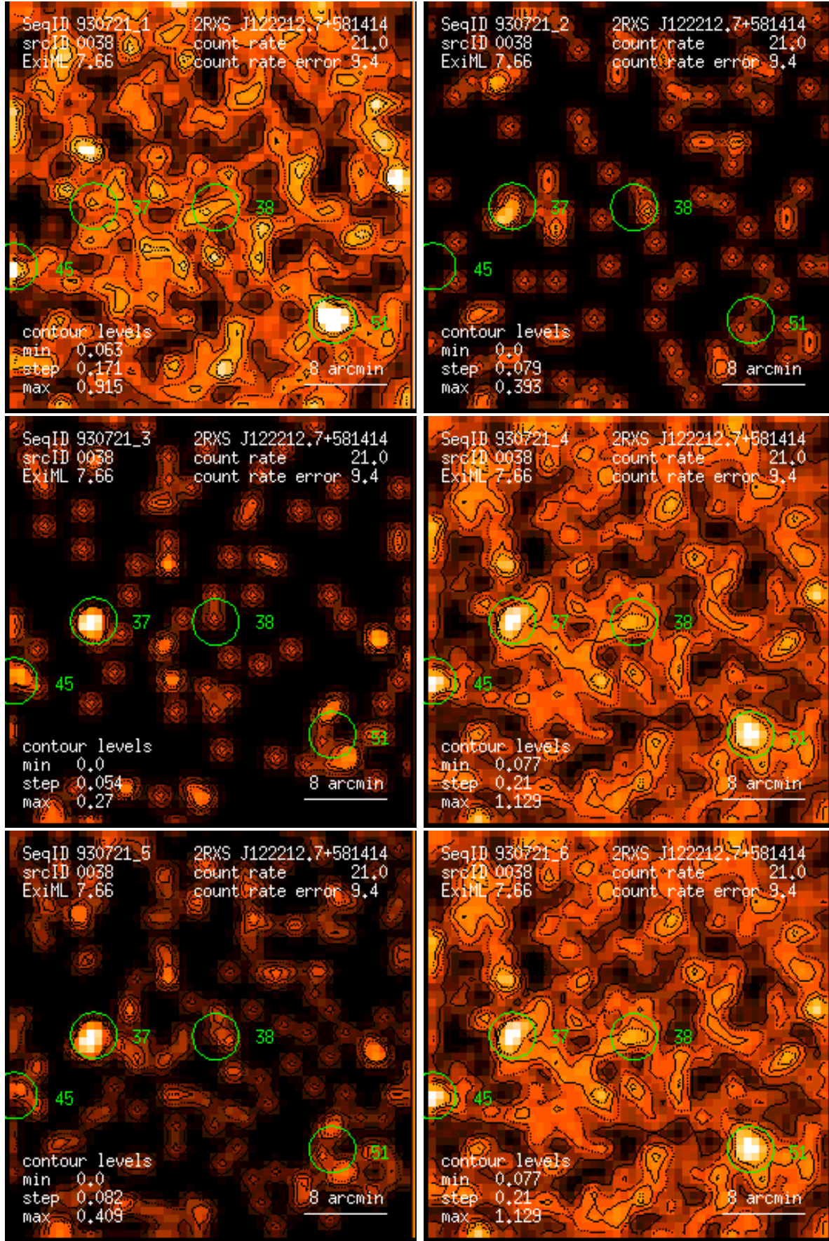
Figure 38: RASS 930721: detection 0038: band rate images, Gaussian filter: (1) PSPC channels 11 – 41, (2) 52 – 90, (3) 91 – 201, (4) 11 – 235, (5) 52 – 201, (6) 11 – 201. Broad band rates in counts/ks. Band rate contour levels in counts/ks/arcmin 2 .
