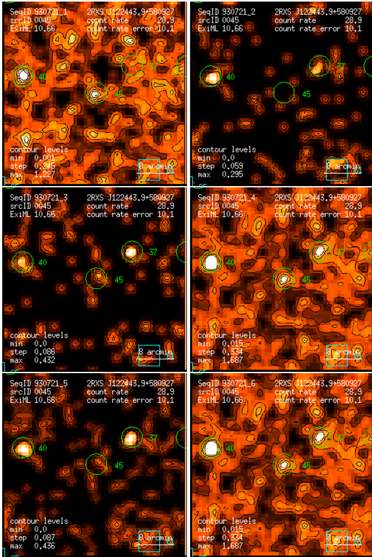
Figure 45: RASS 930721: detection 0045: band rate images, Gaussian filter: (1) PSPC channels 11 – 41, (2) 52 – 90, (3) 91 – 201, (4) 11 – 235, (5) 52 – 201, (6) 11 – 201. Broad band rates in counts/ks. Band rate contour levels in counts/ks/arcmin 2 .
