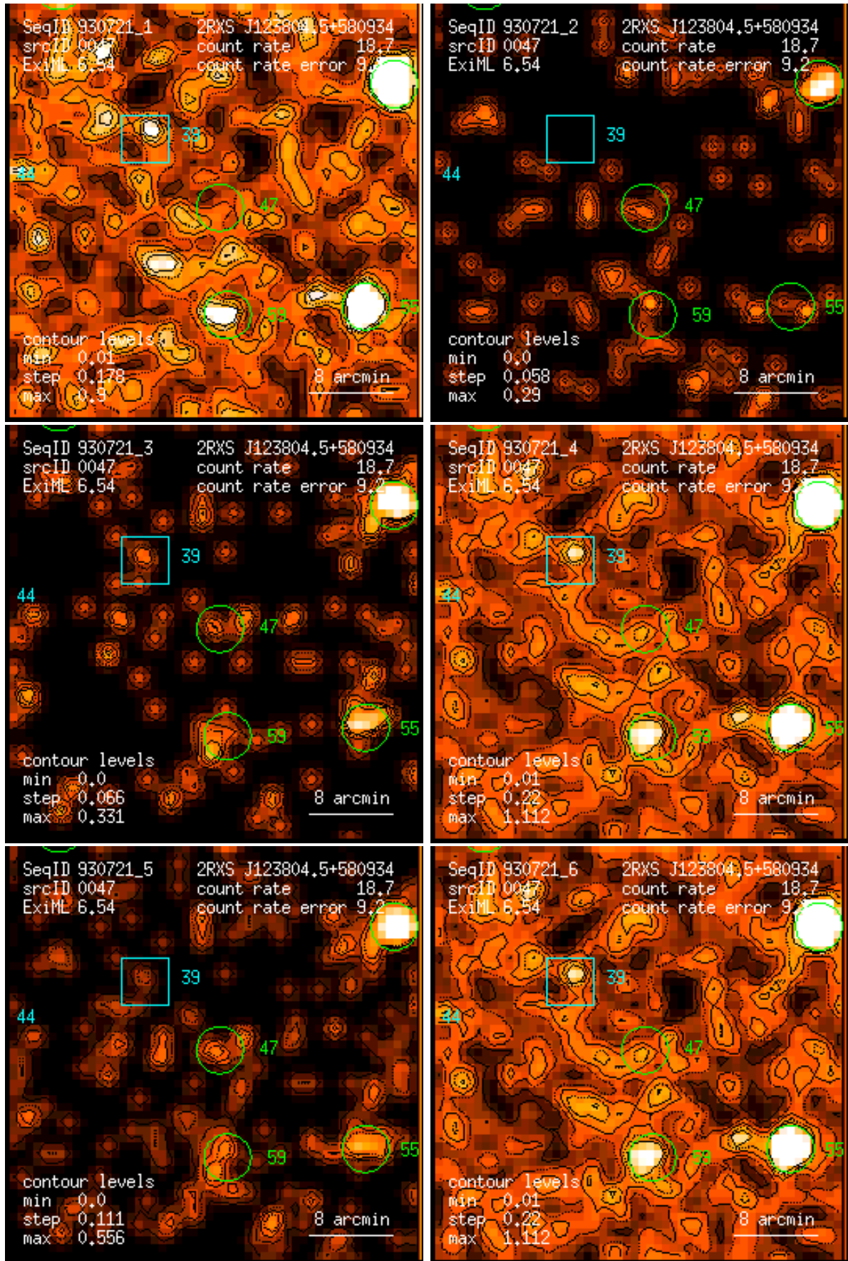
Figure 47: RASS 930721: detection 0047: band rate images, Gaussian filter: (1) PSPC channels 11 – 41, (2) 52 – 90, (3) 91 – 201, (4) 11 – 235, (5) 52 – 201, (6) 11 – 201. Broad band rates in counts/ks. Band rate contour levels in counts/ks/arcmin 2 .
