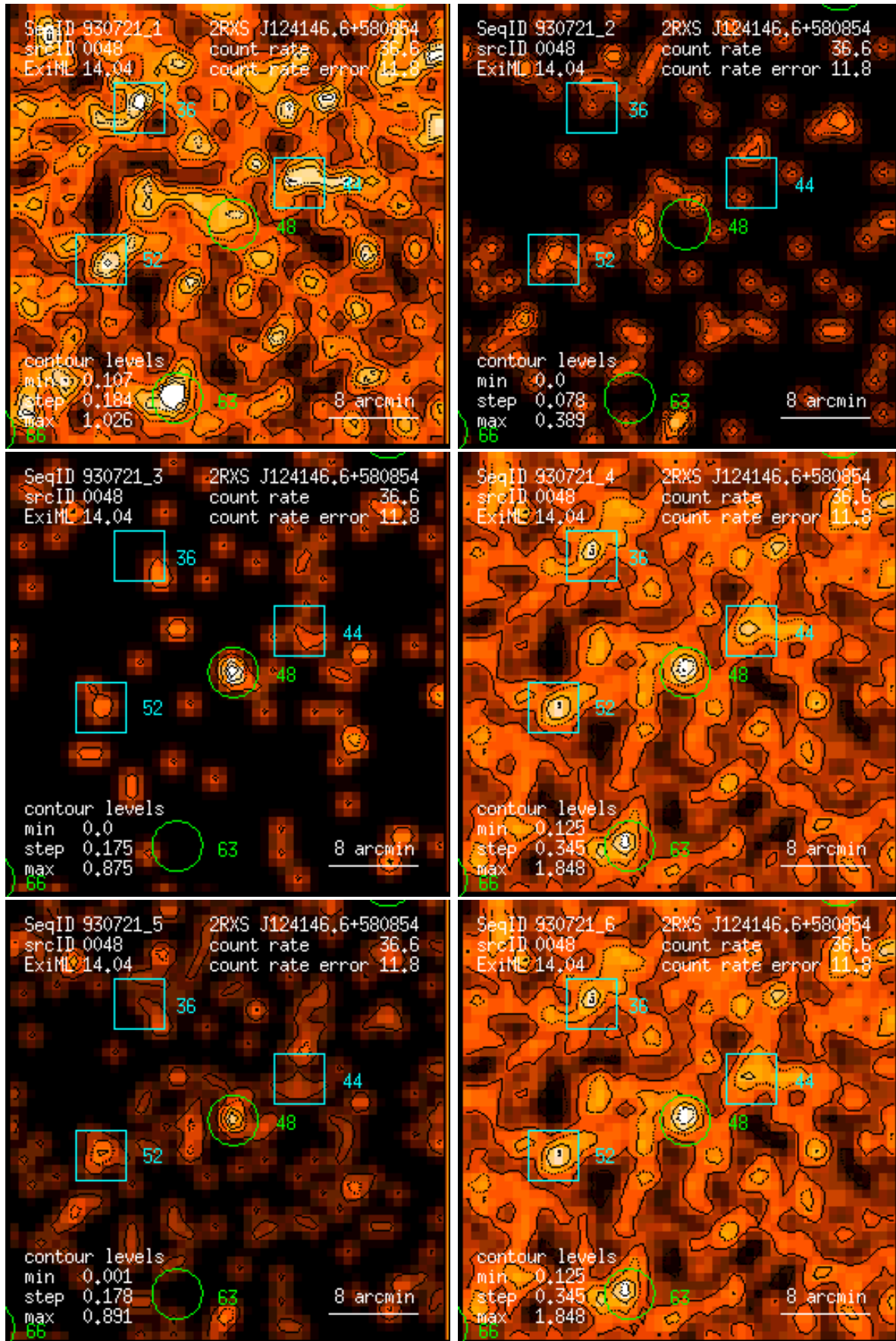
Figure 48: RASS 930721: detection 0048: band rate images, Gaussian filter: (1) PSPC channels 11 – 41, (2) 52 – 90, (3) 91 – 201, (4) 11 – 235, (5) 52 – 201, (6) 11 – 201. Broad band rates in counts/ks. Band rate contour levels in counts/ks/arcmin 2 .
