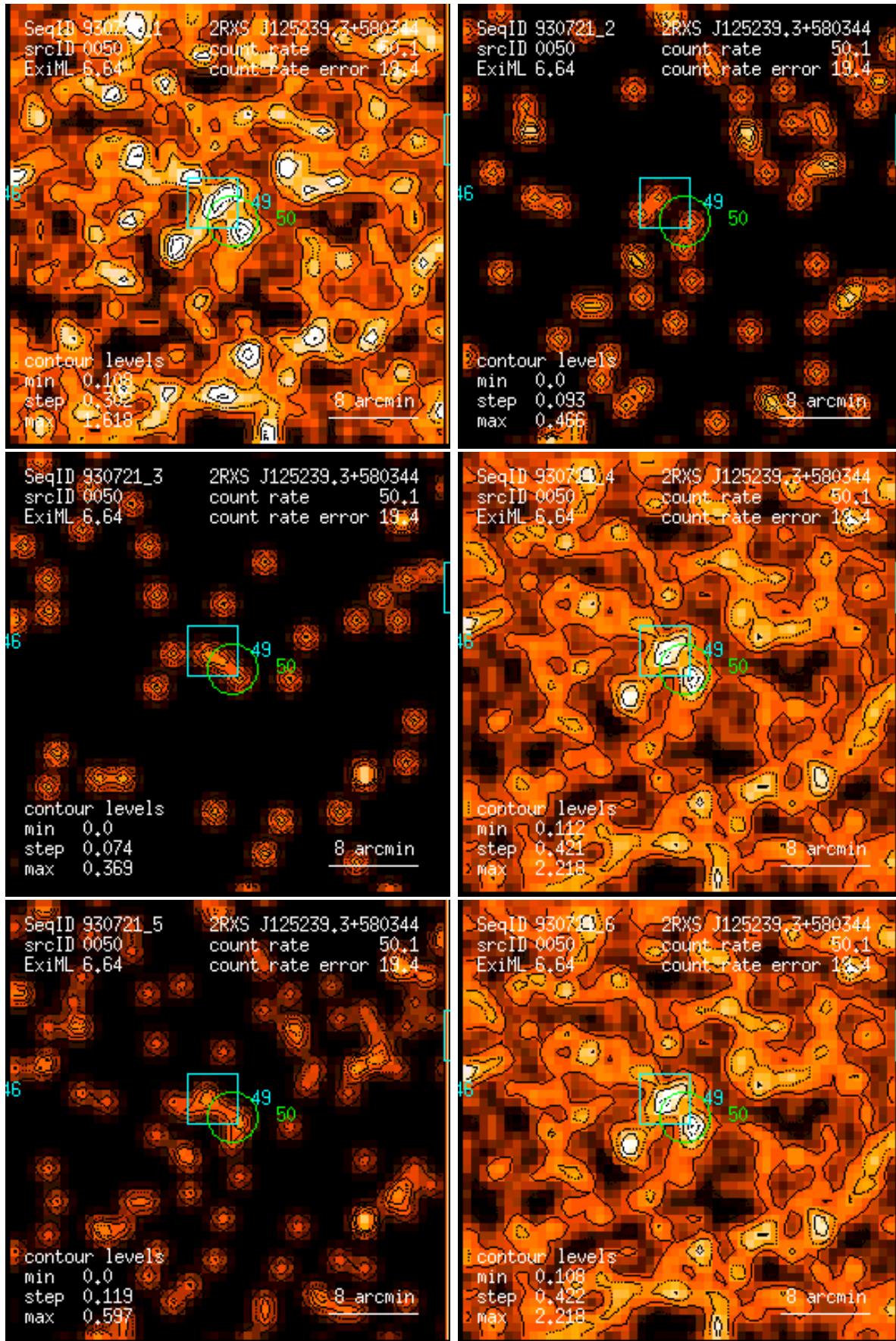
Figure 50: RASS 930721: detection 0050: band rate images, Gaussian filter: (1) PSPC channels 11 – 41, (2) 52 – 90, (3) 91 – 201, (4) 11 – 235, (5) 52 – 201, (6) 11 – 201. Broad band rates in counts/ks. Band rate contour levels in counts/ks/arcmin 2 .
