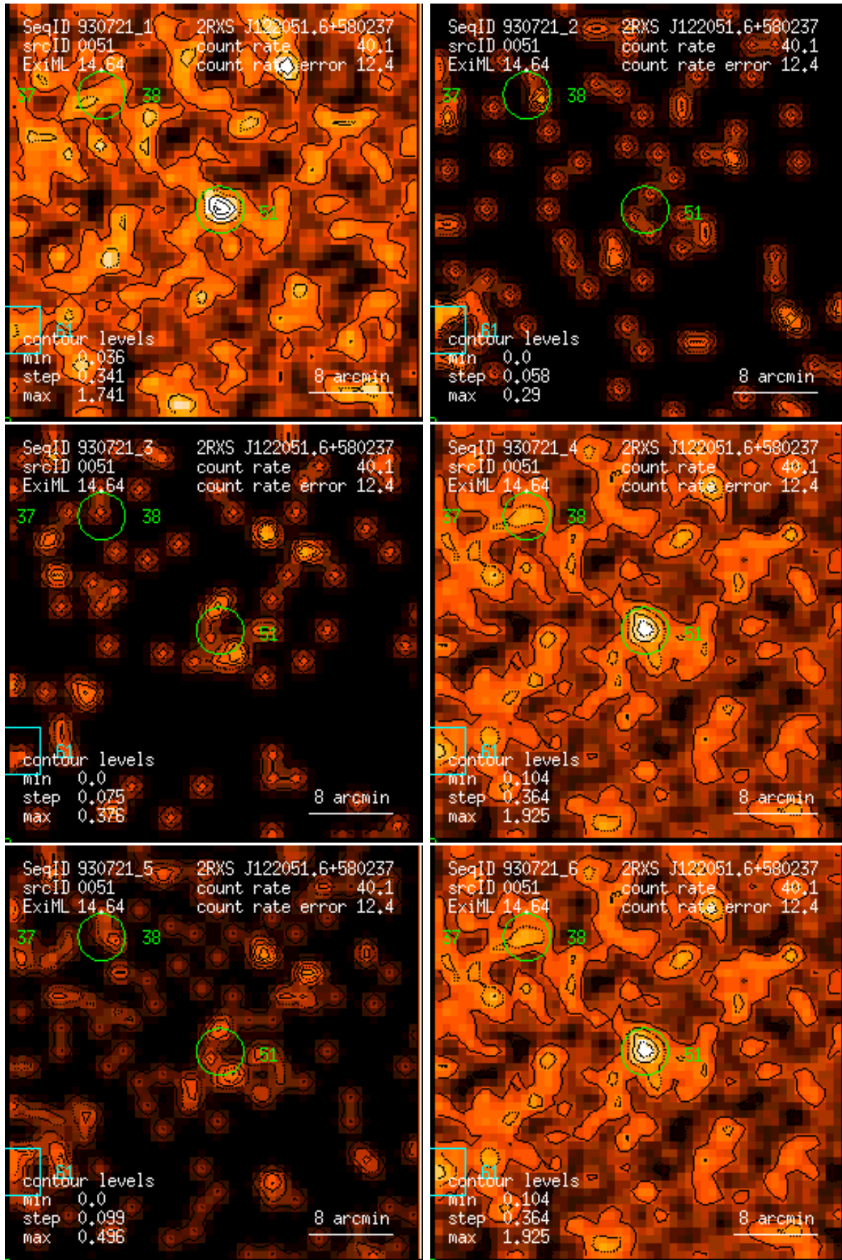
Figure 51: RASS 930721: detection 0051: band rate images, Gaussian filter: (1) PSPC channels 11 – 41, (2) 52 – 90, (3) 91 – 201, (4) 11 – 235, (5) 52 – 201, (6) 11 – 201. Broad band rates in counts/ks. Band rate contour levels in counts/ks/arcmin 2 .
