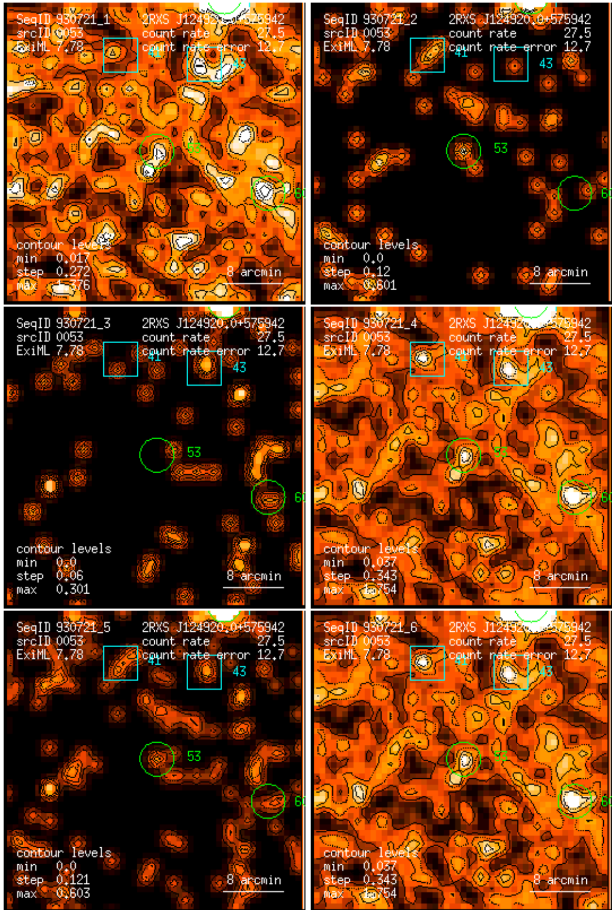
Figure 53: RASS 930721: detection 0053: band rate images, Gaussian filter: (1) PSPC channels 11 – 41, (2) 52 – 90, (3) 91 – 201, (4) 11 – 235, (5) 52 – 201, (6) 11 – 201. Broad band rates in counts/ks. Band rate contour levels in counts/ks/arcmin 2 .
