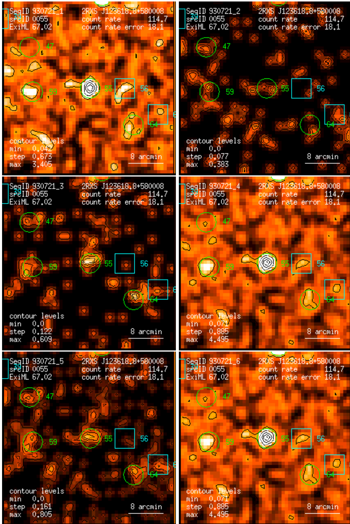
Figure 55: RASS 930721: detection 0055: band rate images, Gaussian filter: (1) PSPC channels 11 – 41, (2) 52 – 90, (3) 91 – 201, (4) 11 – 235, (5) 52 – 201, (6) 11 – 201. Broad band rates in counts/ks. Band rate contour levels in counts/ks/arcmin 2 .
