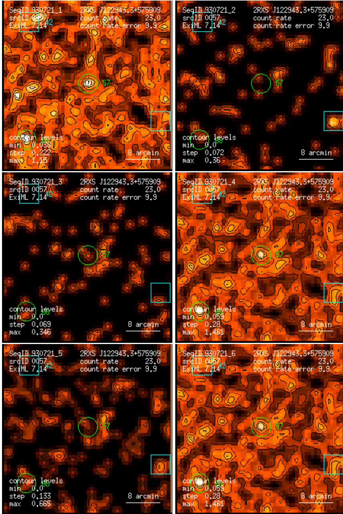
Figure 57: RASS 930721: detection 0057: band rate images, Gaussian filter: (1) PSPC channels 11 – 41, (2) 52 – 90, (3) 91 – 201, (4) 11 – 235, (5) 52 – 201, (6) 11 – 201. Broad band rates in counts/ks. Band rate contour levels in counts/ks/arcmin 2 .
