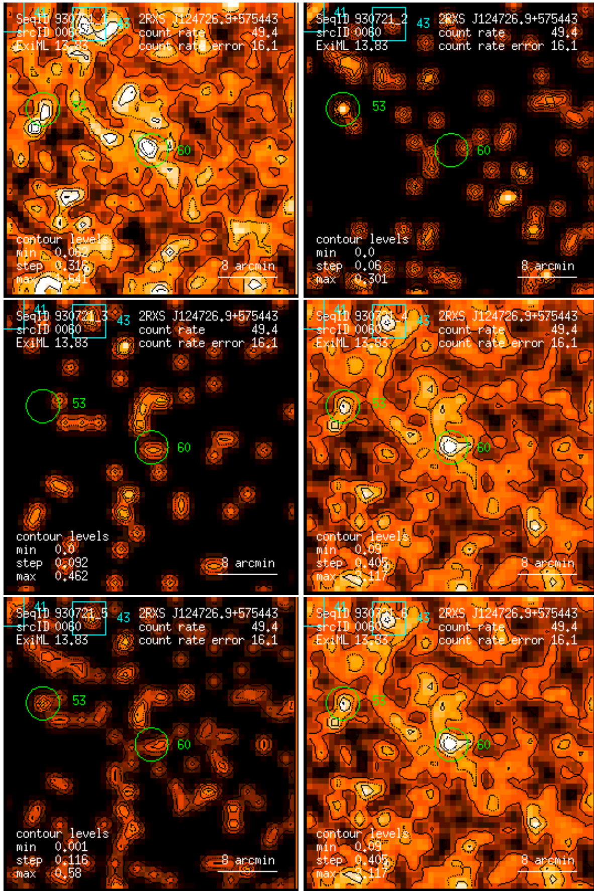
Figure 60: RASS 930721: detection 0060: band rate images, Gaussian filter: (1) PSPC channels 11 – 41, (2) 52 – 90, (3) 91 – 201, (4) 11 – 235, (5) 52 – 201, (6) 11 – 201. Broad band rates in counts/ks. Band rate contour levels in counts/ks/arcmin 2 .
