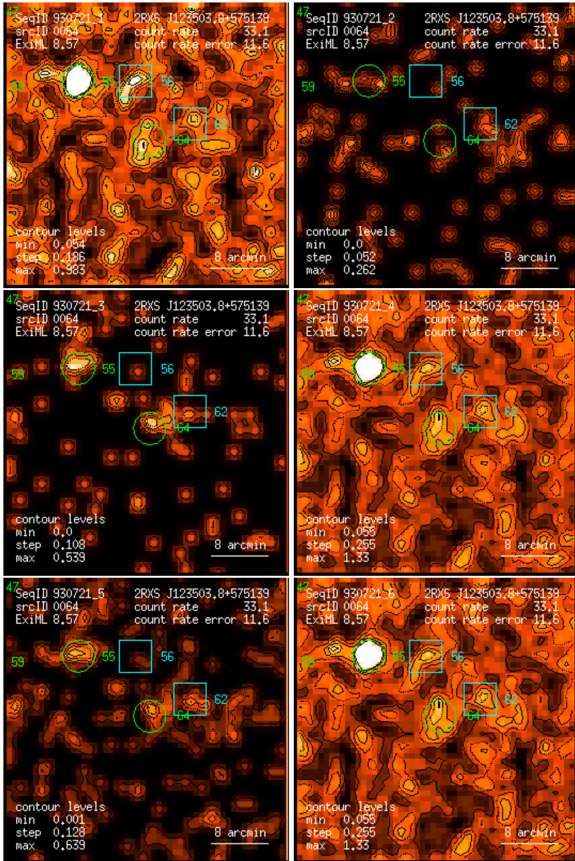
Figure 64: RASS 930721: detection 0064: band rate images, Gaussian filter: (1) PSPC channels 11 – 41, (2) 52 – 90, (3) 91 – 201, (4) 11 – 235, (5) 52 – 201, (6) 11 – 201. Broad band rates in counts/ks. Band rate contour levels in counts/ks/arcmin 2 .
