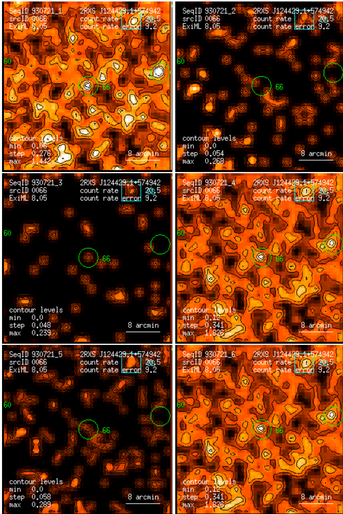
Figure 66: RASS 930721: detection 0066: band rate images, Gaussian filter: (1) PSPC channels 11 – 41, (2) 52 – 90, (3) 91 – 201, (4) 11 – 235, (5) 52 – 201, (6) 11 – 201. Broad band rates in counts/ks. Band rate contour levels in counts/ks/arcmin 2 .
