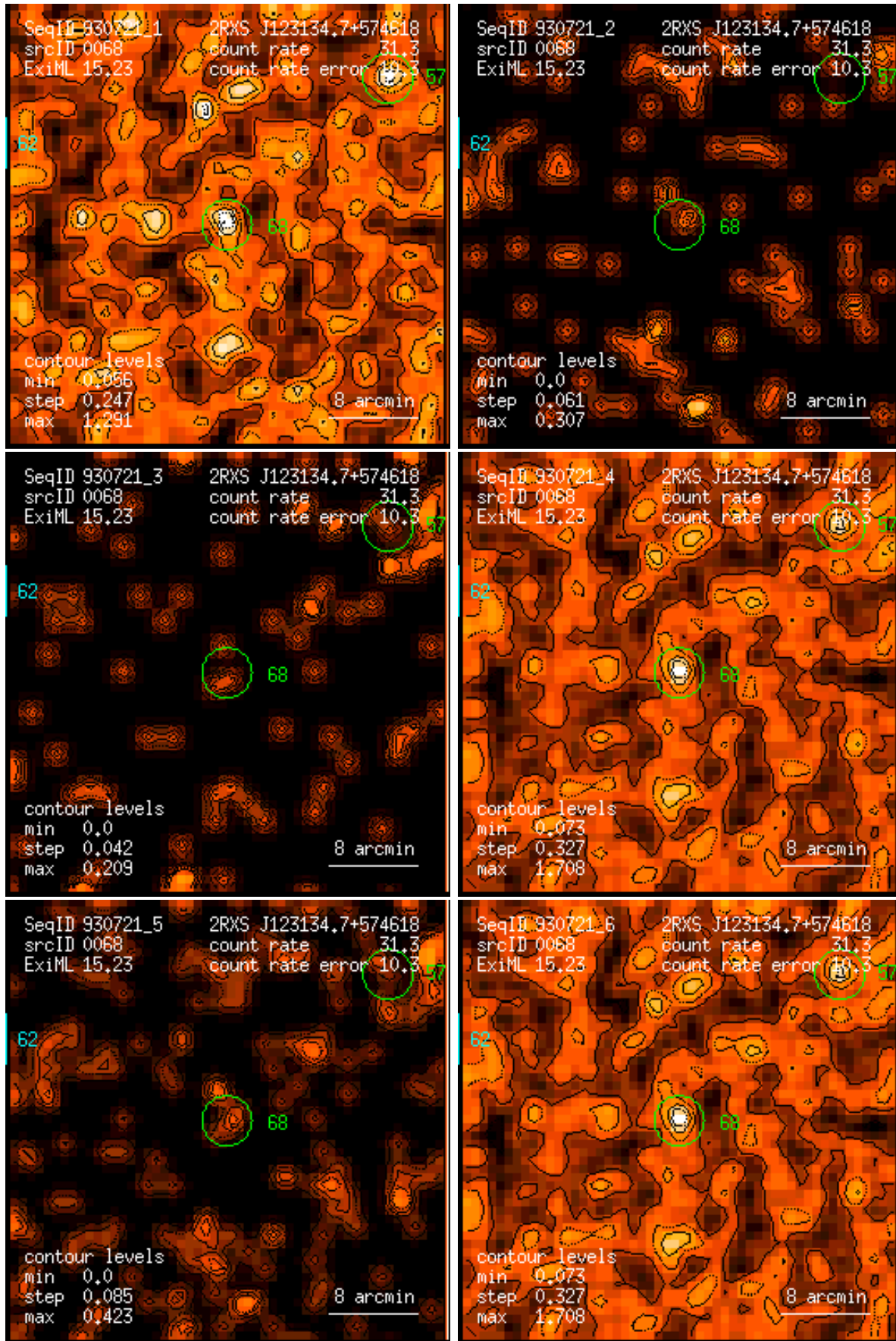
Figure 68: RASS 930721: detection 0068: band rate images, Gaussian filter: (1) PSPC channels 11 – 41, (2) 52 – 90, (3) 91 – 201, (4) 11 – 235, (5) 52 – 201, (6) 11 – 201. Broad band rates in counts/ks. Band rate contour levels in counts/ks/arcmin 2 .
