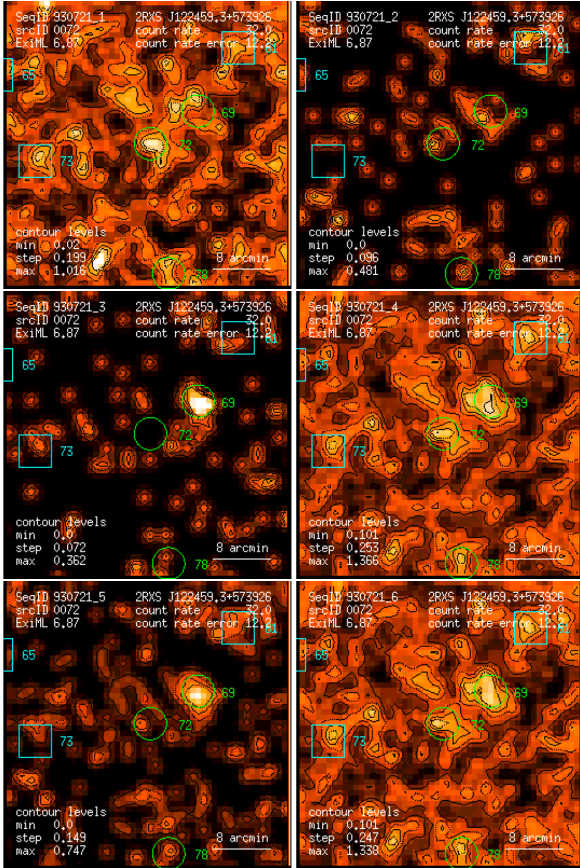
Figure 72: RASS 930721: detection 0072: band rate images, Gaussian filter: (1) PSPC channels 11 – 41, (2) 52 – 90, (3) 91 – 201, (4) 11 – 235, (5) 52 – 201, (6) 11 – 201. Broad band rates in counts/ks. Band rate contour levels in counts/ks/arcmin 2 .
