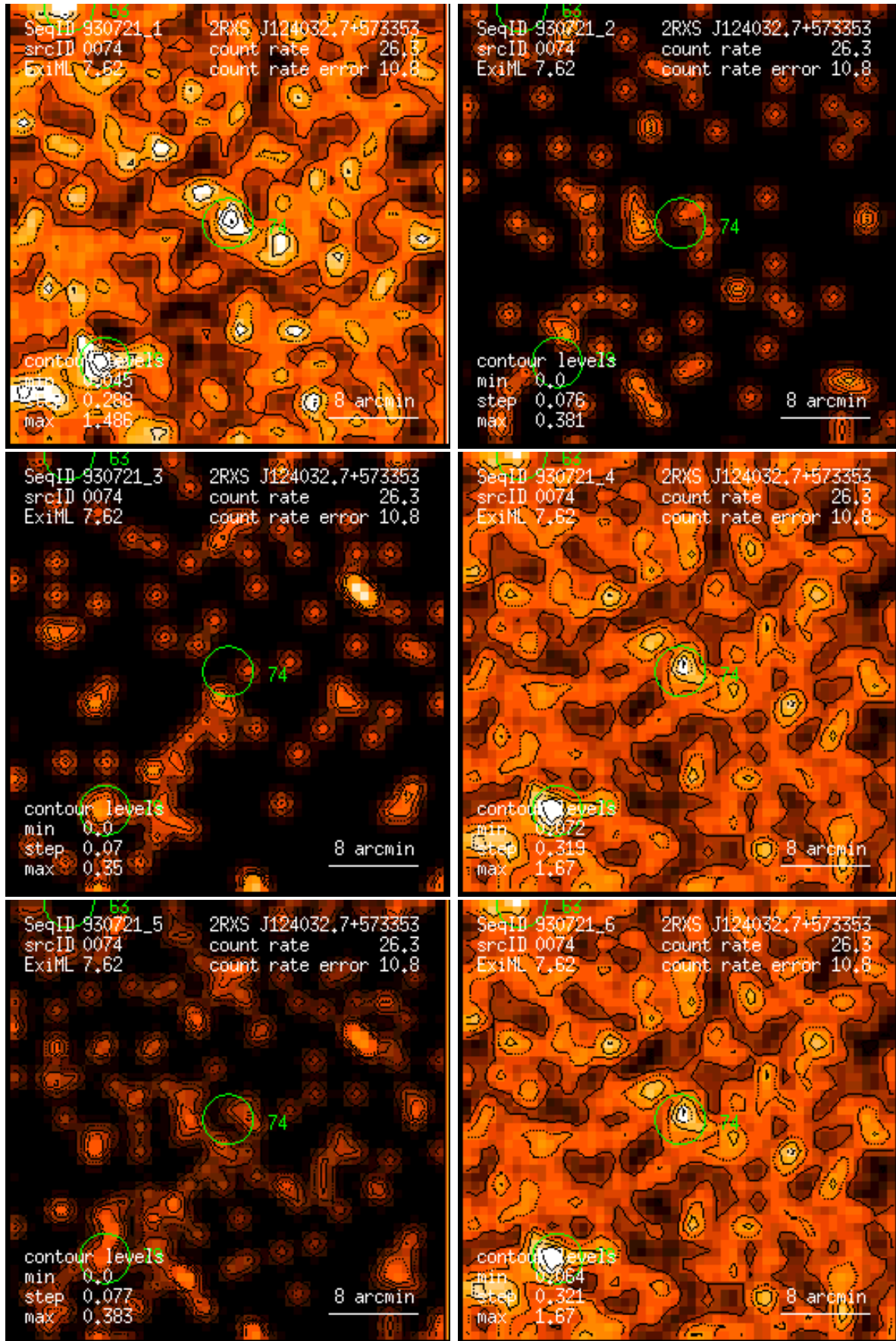
Figure 74: RASS 930721: detection 0074: band rate images, Gaussian filter: (1) PSPC channels 11 – 41, (2) 52 – 90, (3) 91 – 201, (4) 11 – 235, (5) 52 – 201, (6) 11 – 201. Broad band rates in counts/ks. Band rate contour levels in counts/ks/arcmin 2 .
