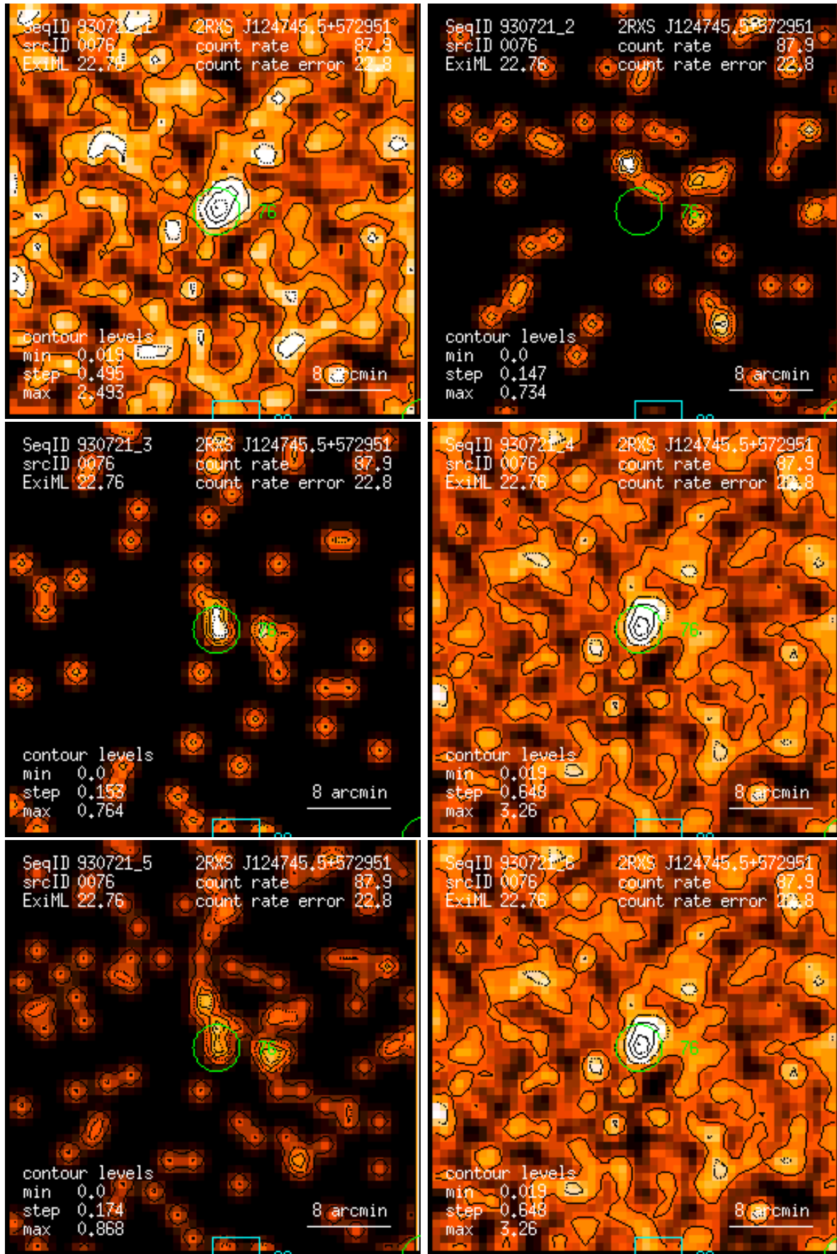
Figure 76: RASS 930721: detection 0076: band rate images, Gaussian filter: (1) PSPC channels 11 – 41, (2) 52 – 90, (3) 91 – 201, (4) 11 – 235, (5) 52 – 201, (6) 11 – 201. Broad band rates in counts/ks. Band rate contour levels in counts/ks/arcmin 2 .
