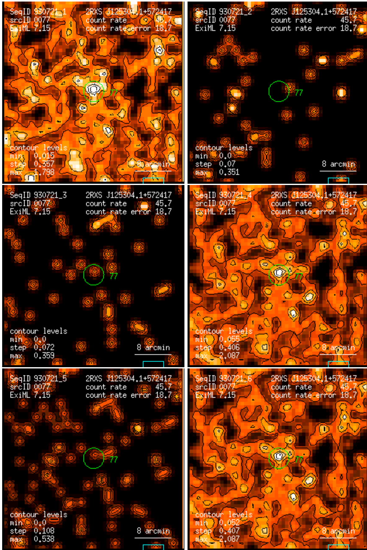
Figure 77: RASS 930721: detection 0077: band rate images, Gaussian filter: (1) PSPC channels 11 – 41, (2) 52 – 90, (3) 91 – 201, (4) 11 – 235, (5) 52 – 201, (6) 11 – 201. Broad band rates in counts/ks. Band rate contour levels in counts/ks/arcmin 2 .
