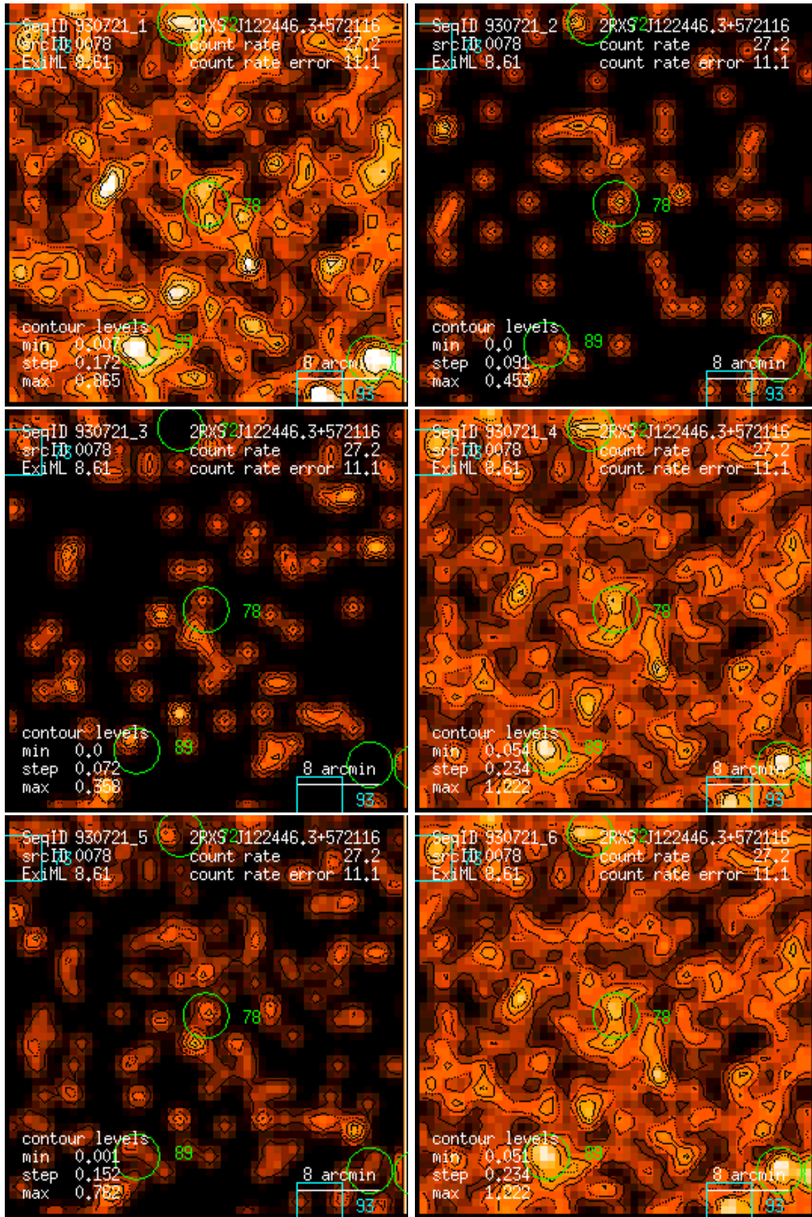
Figure 78: RASS 930721: detection 0078: band rate images, Gaussian filter: (1) PSPC channels 11 – 41, (2) 52 – 90, (3) 91 – 201, (4) 11 – 235, (5) 52 – 201, (6) 11 – 201. Broad band rates in counts/ks. Band rate contour levels in counts/ks/arcmin 2 .
