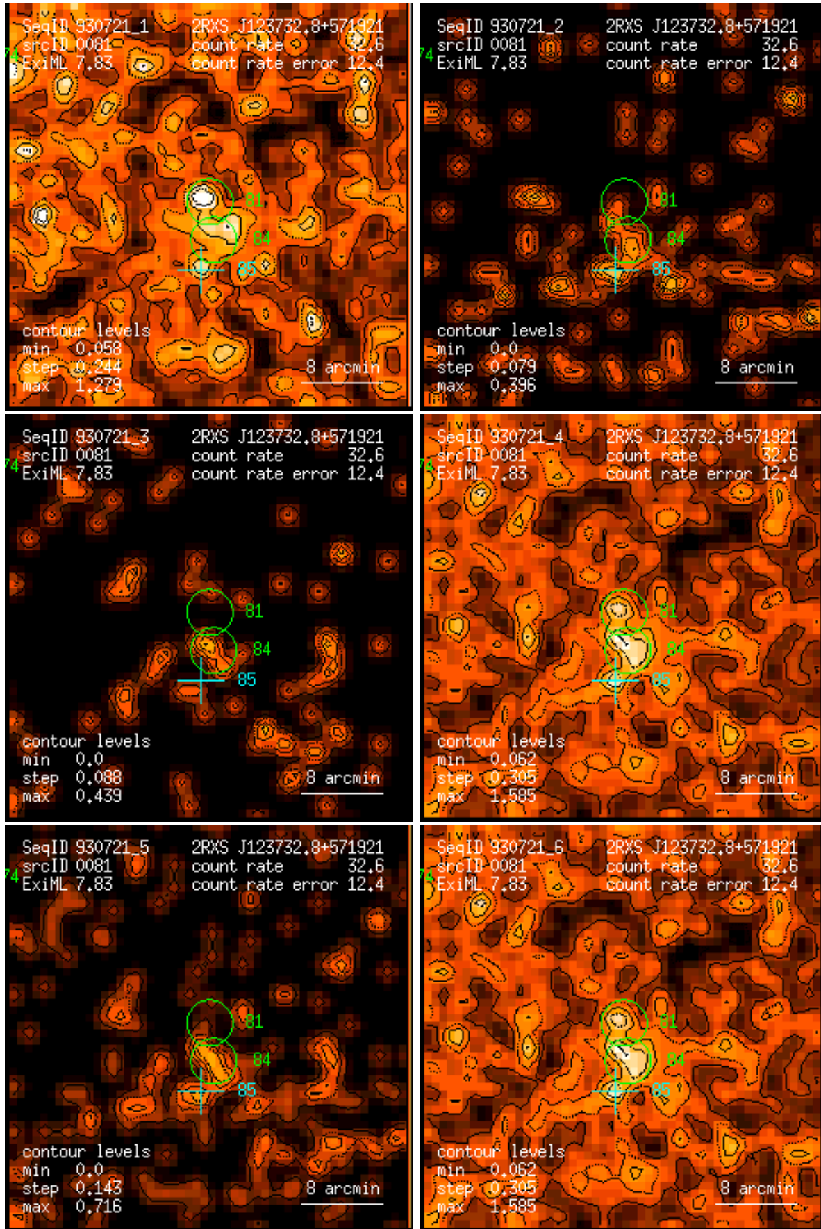
Figure 81: RASS 930721: detection 0081: band rate images, Gaussian filter: (1) PSPC channels 11 – 41, (2) 52 – 90, (3) 91 – 201, (4) 11 – 235, (5) 52 – 201, (6) 11 – 201. Broad band rates in counts/ks. Band rate contour levels in counts/ks/arcmin 2 .
